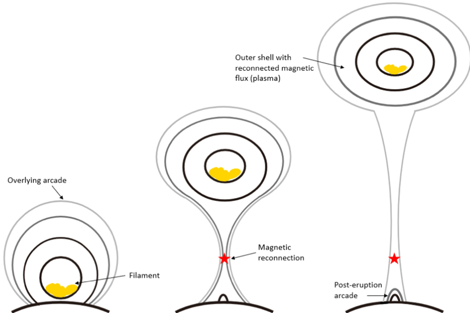
Figure 5. from Bin Zhuang et al 2022 Astrophys. J. 933 doi:10.3847/1538-4357/ac75d4 https://dx.doi.org/10.3847/1538-4357/ac75d4 © 2022. The Author(s). Published by the American Astronomical Society.
