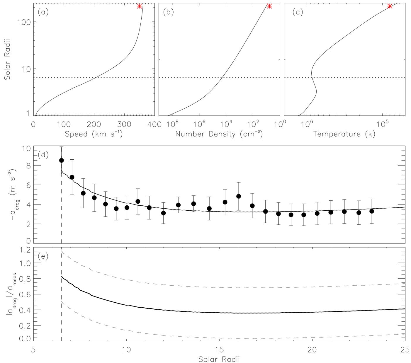
Figure 4. from Bin Zhuang et al 2022 Astrophys. J. 933 doi:10.3847/1538-4357/ac75d4 https://dx.doi.org/10.3847/1538-4357/ac75d4 © 2022. The Author(s). Published by the American Astronomical Society.
