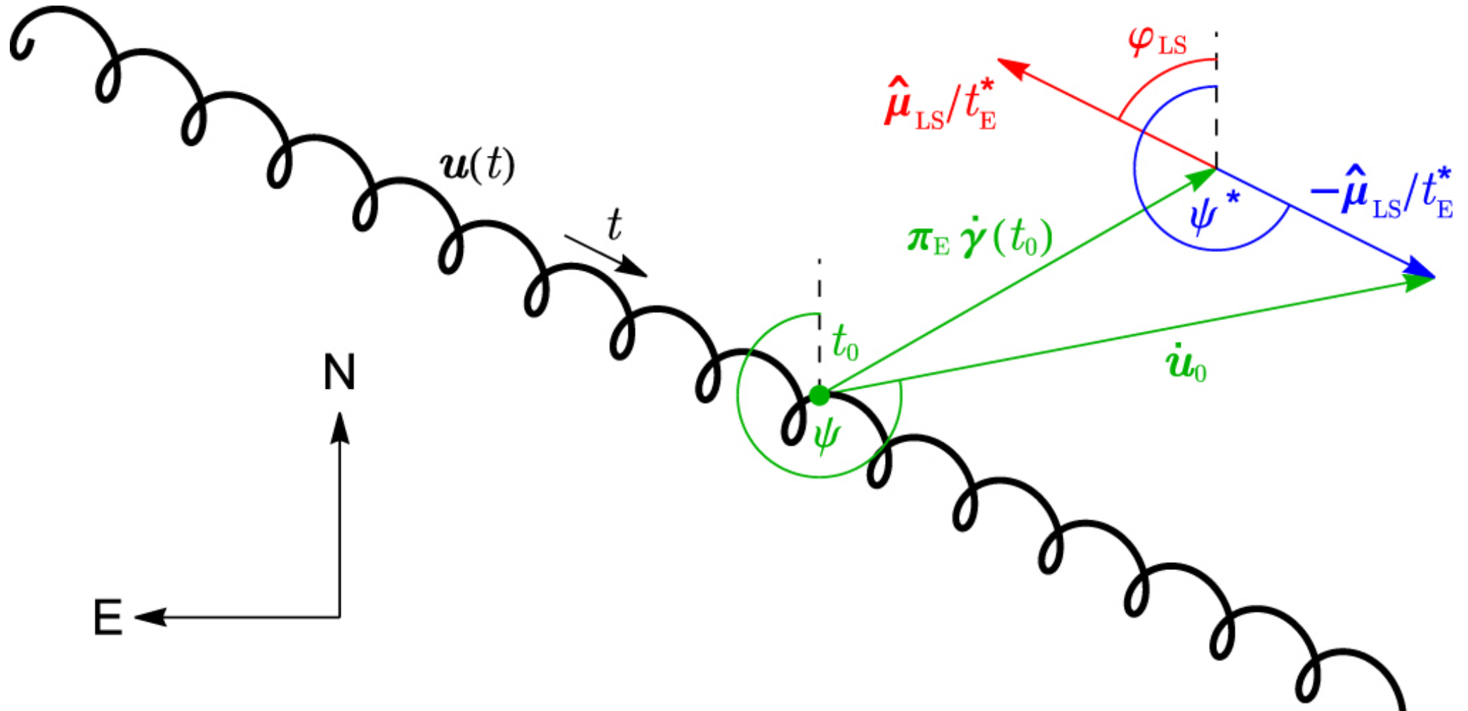
Figure 1. from Kailash C. Sahu et al 2022 Astrophys. J. 933 doi:10.3847/1538-4357/ac739e https://dx.doi.org/10.3847/1538-4357/ac739e © 2022. The Author(s). Published by the American Astronomical Society.
