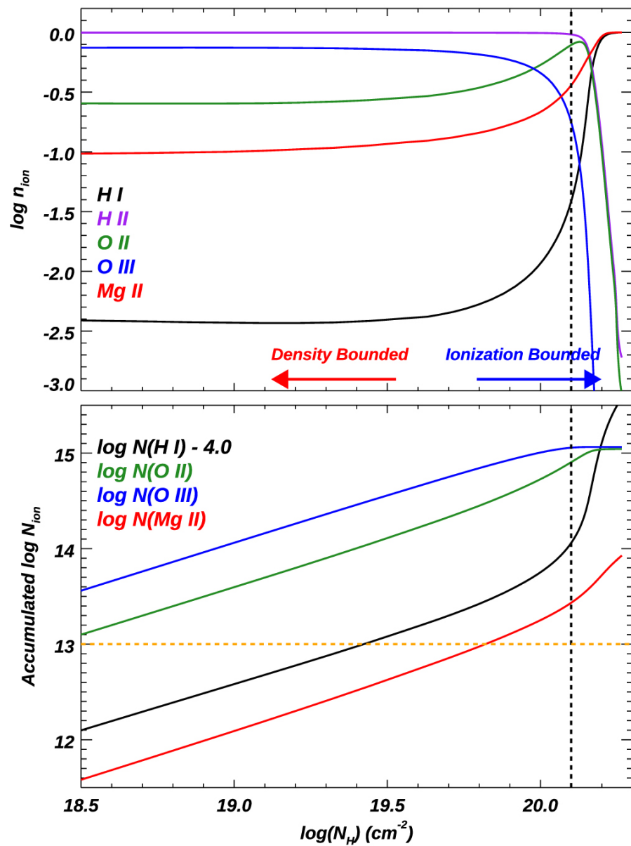
Figure 7. from Xinfeng Xu et al 2022 Astrophys. J. 933 doi:10.3847/1538-4357/ac7225 https://dx.doi.org/10.3847/1538-4357/ac7225 © 2022. The Author(s). Published by the American Astronomical Society.
