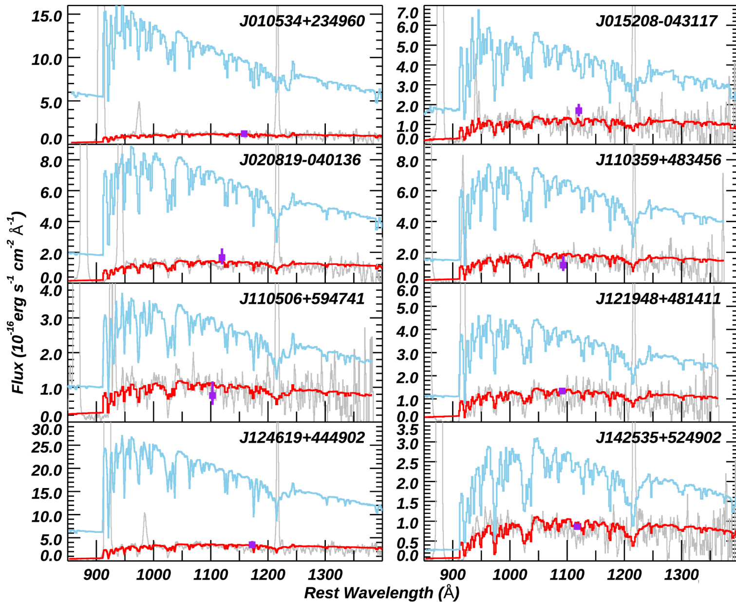
Figure 4. from Xinfeng Xu et al 2022 Astrophys. J. 933 doi:10.3847/1538-4357/ac7225 https://dx.doi.org/10.3847/1538-4357/ac7225 © 2022. The Author(s). Published by the American Astronomical Society.
