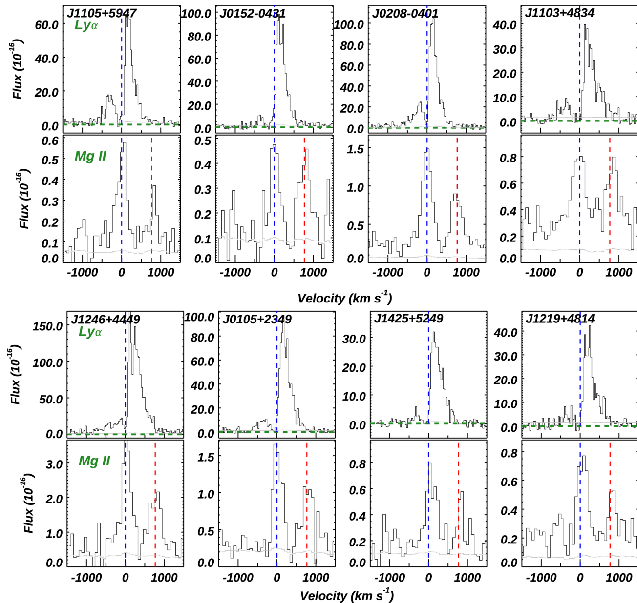
Figure 3. from Xinfeng Xu et al 2022 Astrophys. J. 933 doi:10.3847/1538-4357/ac7225 https://dx.doi.org/10.3847/1538-4357/ac7225 © 2022. The Author(s). Published by the American Astronomical Society.
