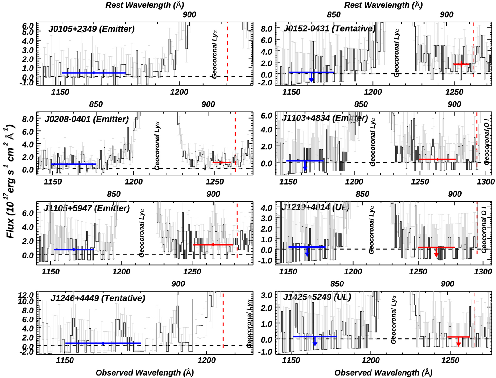
Figure 2. from Xinfeng Xu et al 2022 Astrophys. J. 933 doi:10.3847/1538-4357/ac7225 https://dx.doi.org/10.3847/1538-4357/ac7225 © 2022. The Author(s). Published by the American Astronomical Society.
