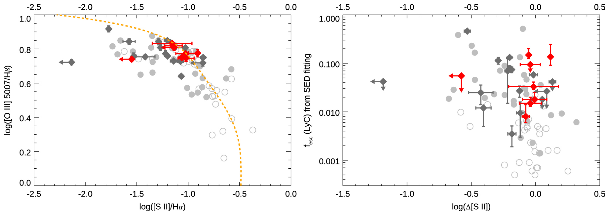
Figure 14. from Xinfeng Xu et al 2022 Astrophys. J. 933 doi:10.3847/1538-4357/ac7225 https://dx.doi.org/10.3847/1538-4357/ac7225 © 2022. The Author(s). Published by the American Astronomical Society.
