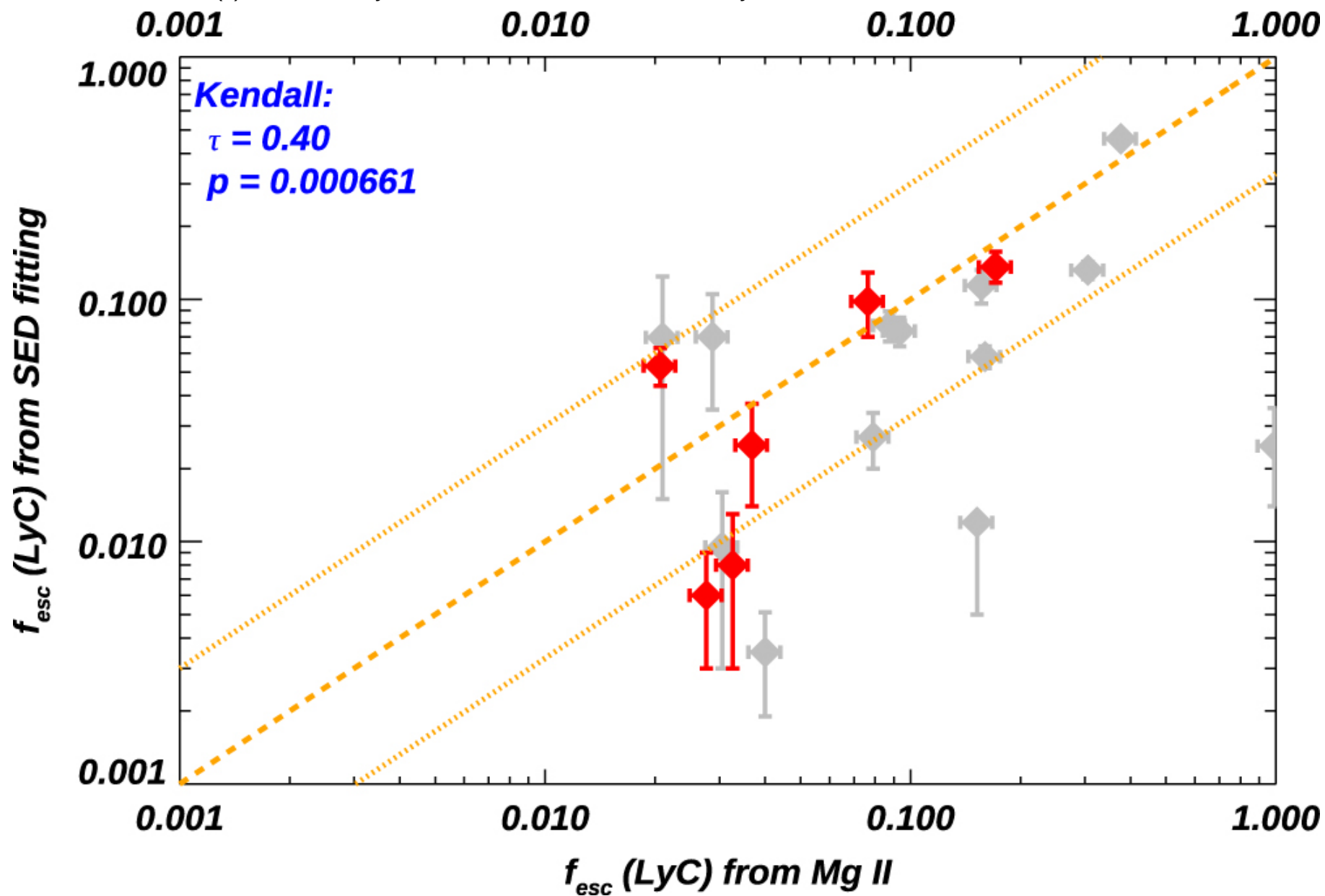
Figure 13. from Xinfeng Xu et al 2022 Astrophys. J. 933 doi:10.3847/1538-4357/ac7225 https://dx.doi.org/10.3847/1538-4357/ac7225 © 2022. The Author(s). Published by the American Astronomical Society.
