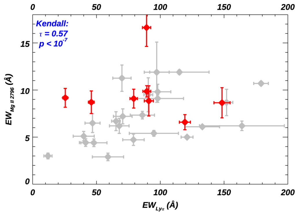
Figure 11. from Xinfeng Xu et al 2022 Astrophys. J. 933 doi:10.3847/1538-4357/ac7225 https://dx.doi.org/10.3847/1538-4357/ac7225 © 2022. The Author(s). Published by the American Astronomical Society.
