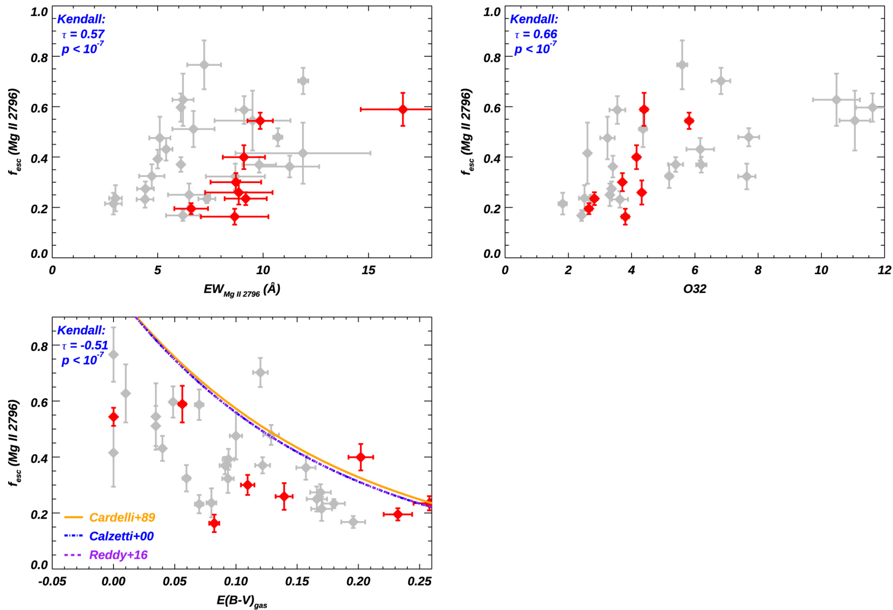
Figure 10. from Xinfeng Xu et al 2022 Astrophys. J. 933 doi:10.3847/1538-4357/ac7225 https://dx.doi.org/10.3847/1538-4357/ac7225 © 2022. The Author(s). Published by the American Astronomical Society.
