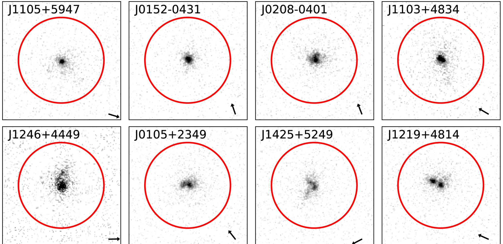
Figure 1. from Xinfeng Xu et al 2022 Astrophys. J. 933 doi:10.3847/1538-4357/ac7225 https://dx.doi.org/10.3847/1538-4357/ac7225 © 2022. The Author(s). Published by the American Astronomical Society.
