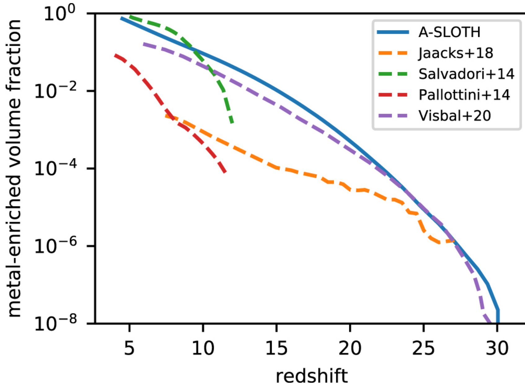
Figure 9. from Tilman Hartwig et al 2022 Astrophys. J. 936 doi:10.3847/1538-4357/ac7150 https://dx.doi.org/10.3847/1538-4357/ac7150 © 2022. The Author(s). Published by the American Astronomical Society.
