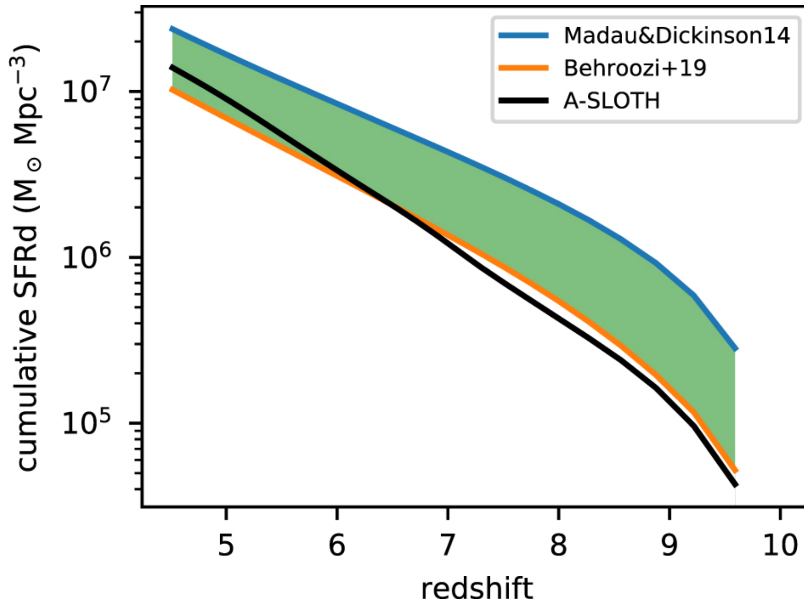
Figure 7. from Tilman Hartwig et al 2022 Astrophys. J. 936 doi:10.3847/1538-4357/ac7150 https://dx.doi.org/10.3847/1538-4357/ac7150 © 2022. The Author(s). Published by the American Astronomical Society.
