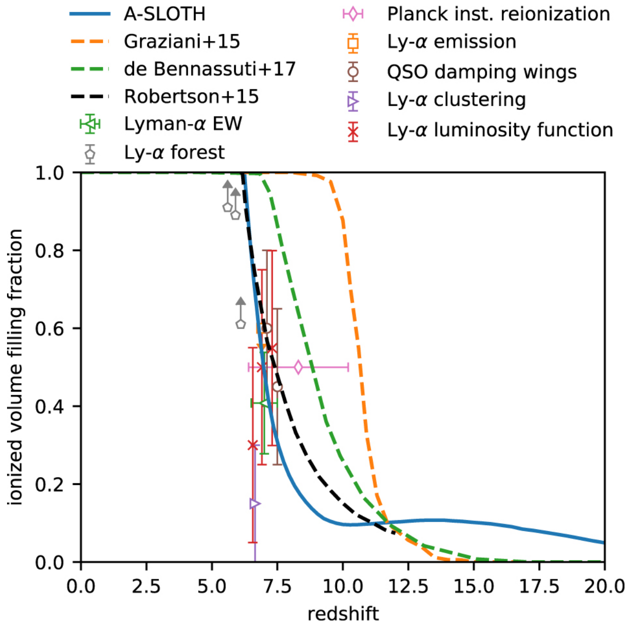
Figure 5. from Tilman Hartwig et al 2022 Astrophys. J. 936 doi:10.3847/1538-4357/ac7150 https://dx.doi.org/10.3847/1538-4357/ac7150
