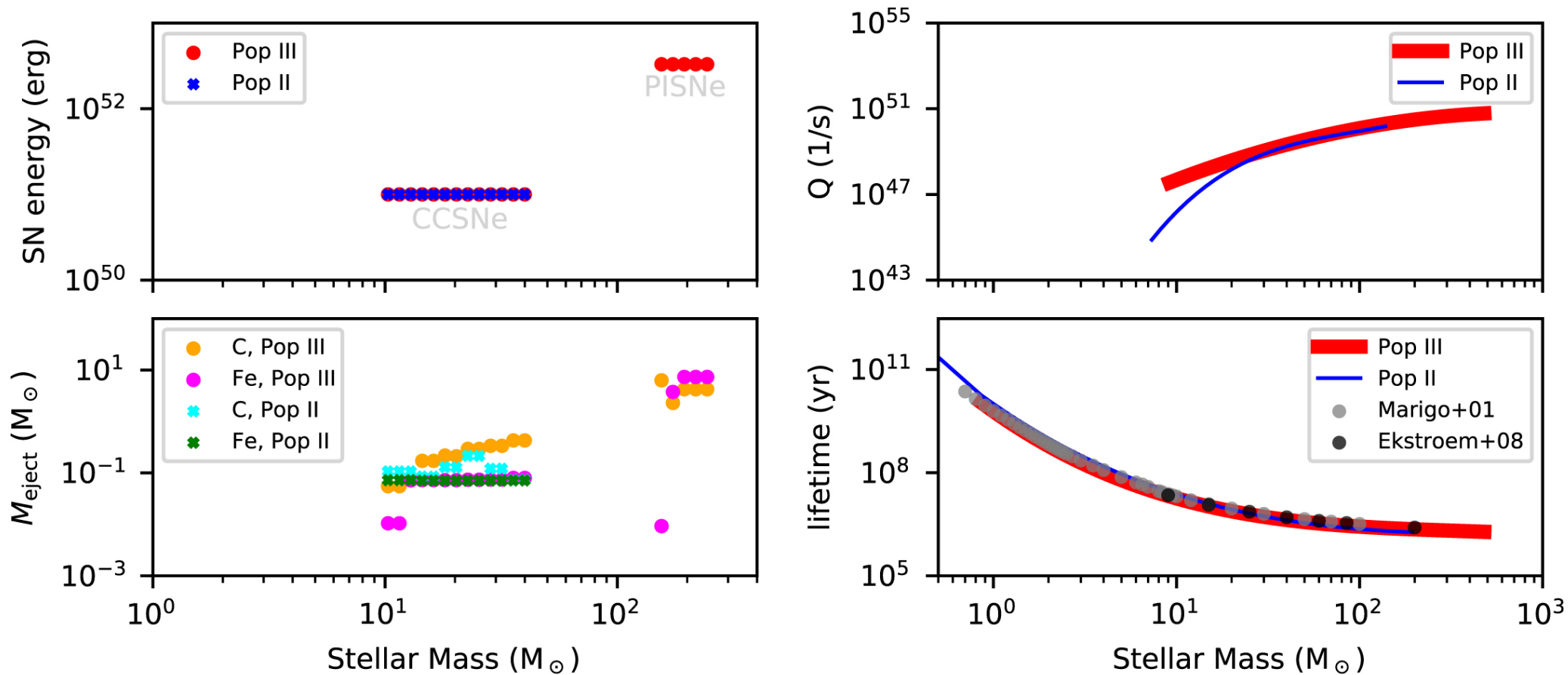
Figure 2. from Tilman Hartwig et al 2022 Astrophys. J. 936 doi:10.3847/1538-4357/ac7150 https://dx.doi.org/10.3847/1538-4357/ac7150 © 2022. The Author(s). Published by the American Astronomical Society.
