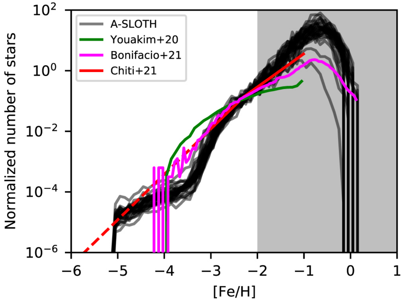
Figure 11. from Tilman Hartwig et al 2022 Astrophys. J. 936 doi:10.3847/1538-4357/ac7150 https://dx.doi.org/10.3847/1538-4357/ac7150 © 2022. The Author(s). Published by the American Astronomical Society.
