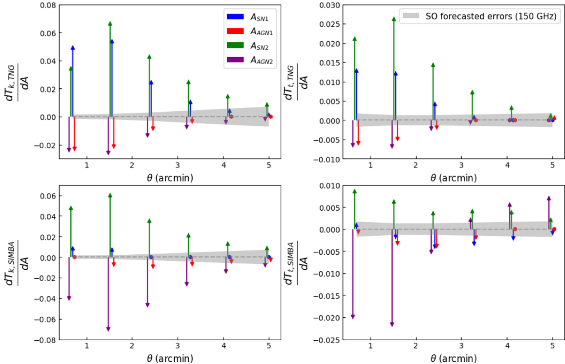
Figure 4. from Emily Moser et al 2022 Astrophys. J. 933 doi:10.3847/1538-4357/ac70c6 https://dx.doi.org/10.3847/1538-4357/ac70c6 © 2022. The Author(s). Published by the American Astronomical Society.
