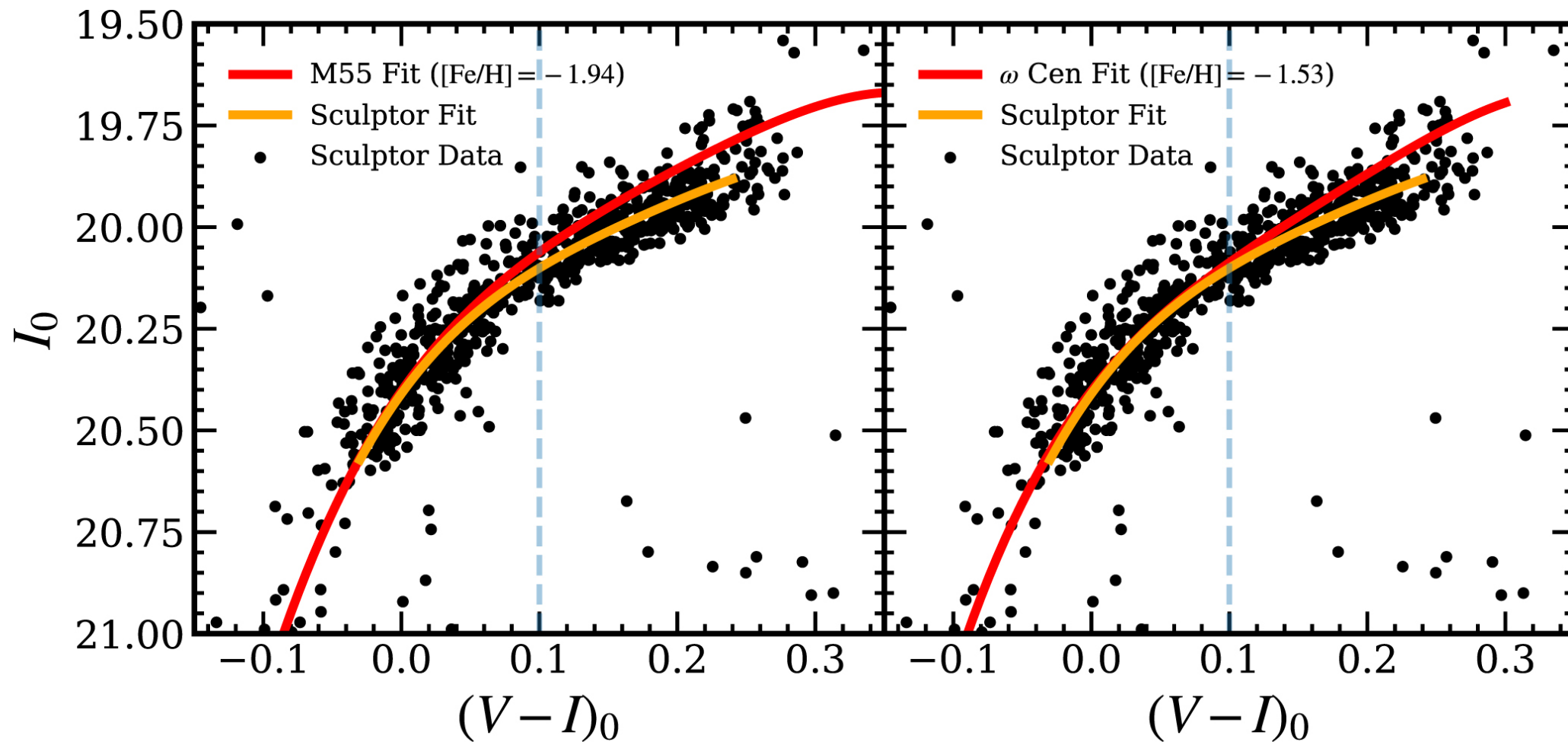
Figure 8. from Quang H. Tran et al 2022 Astrophys. J. 935 doi:10.3847/1538-4357/ac6fe0 https://dx.doi.org/10.3847/1538-4357/ac6fe0 © 2022. The Author(s). Published by the American Astronomical Society.
