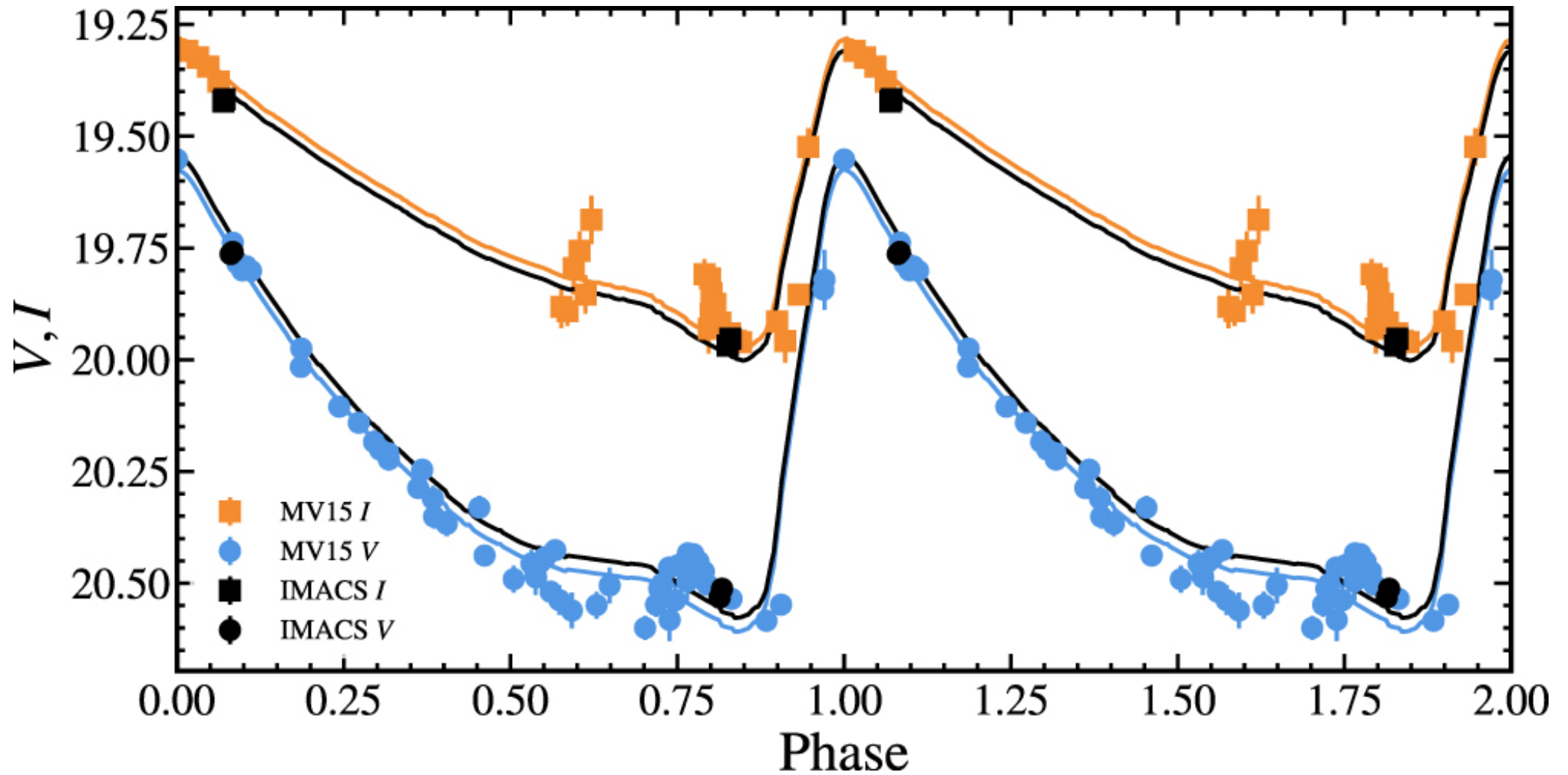
Figure 5. from Quang H. Tran et al 2022 Astrophys. J. 935 doi:10.3847/1538-4357/ac6fe0 https://dx.doi.org/10.3847/1538-4357/ac6fe0 © 2022. The Author(s). Published by the American Astronomical Society.
