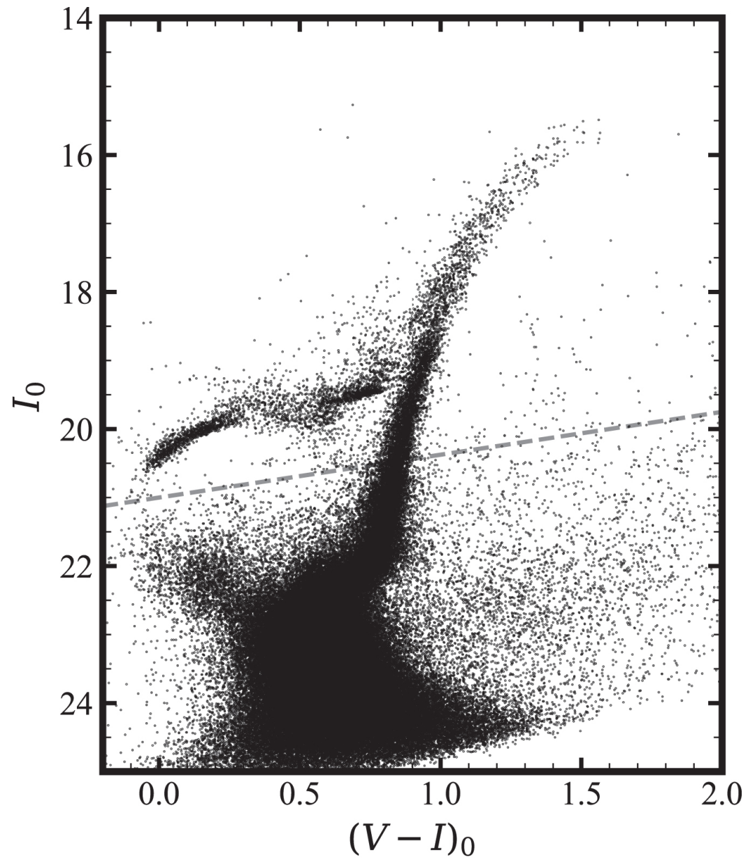
Figure 3. from Quang H. Tran et al 2022 Astrophys. J. 935 doi:10.3847/1538-4357/ac6fe0 https://dx.doi.org/10.3847/1538-4357/ac6fe0 © 2022. The Author(s). Published by the American Astronomical Society.
