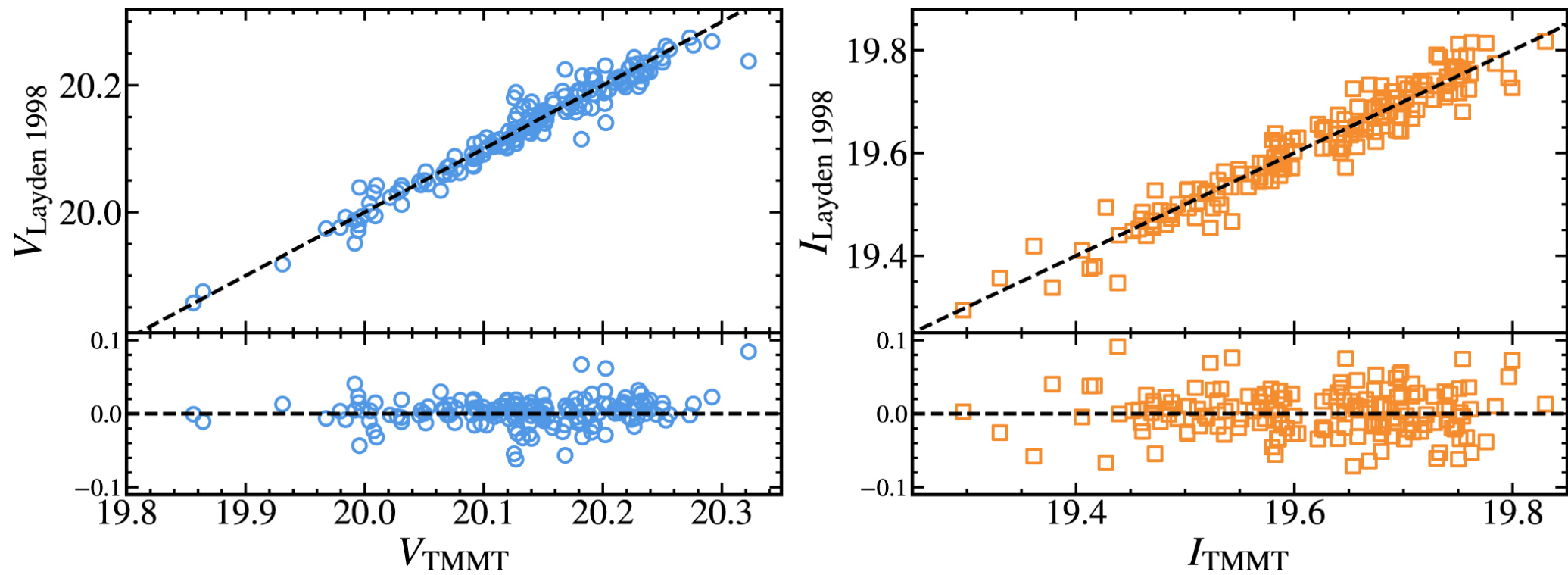
Figure B1. from Quang H. Tran et al 2022 Astrophys. J. 935 doi:10.3847/1538-4357/ac6fe0 https://dx.doi.org/10.3847/1538-4357/ac6fe0 © 2022. The Author(s). Published by the American Astronomical Society.
