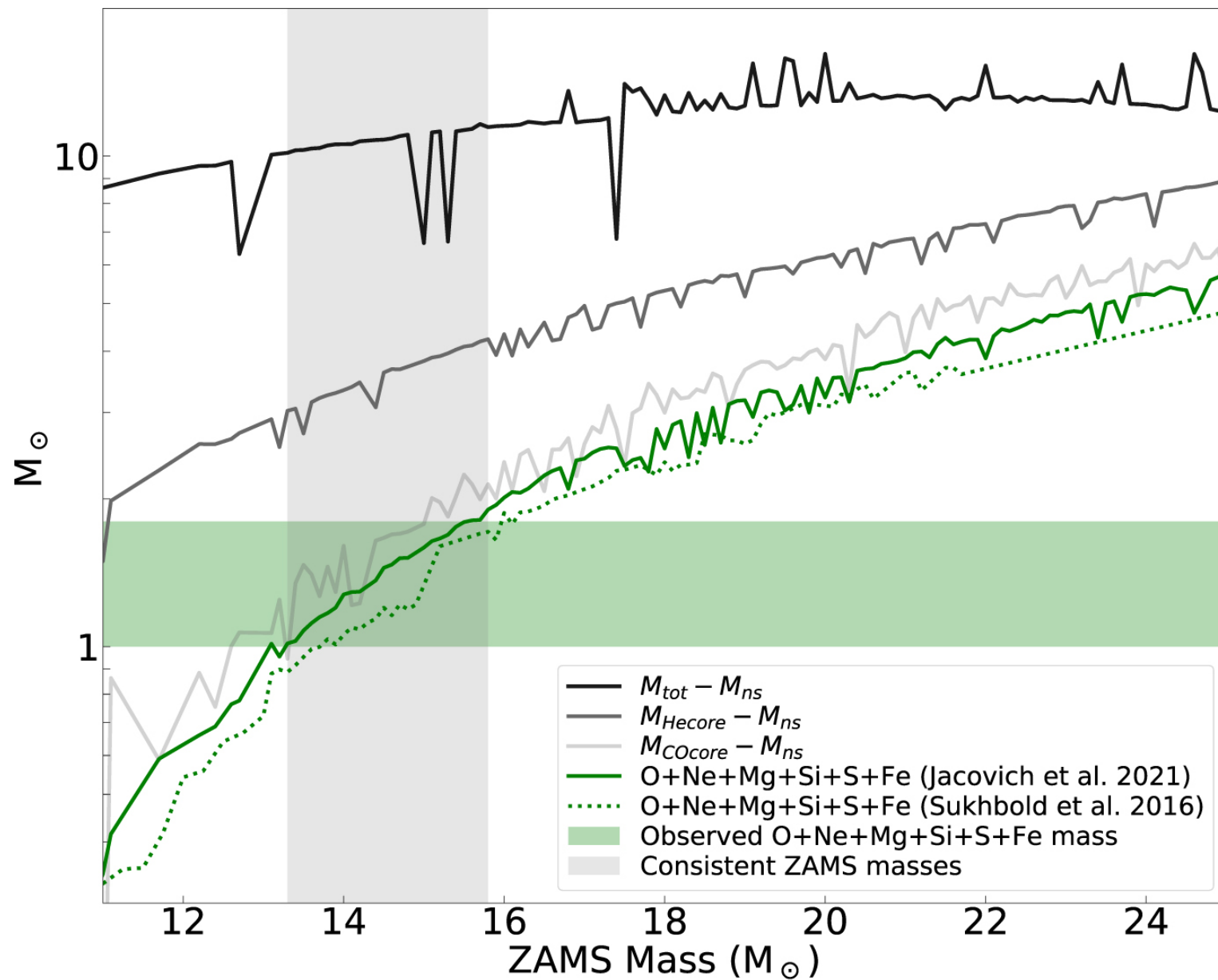
Figure 8. from Tea Temim et al 2022 Astrophys. J. 932 doi:10.3847/1538-4357/ac6bf4 https://dx.doi.org/10.3847/1538-4357/ac6bf4 © 2022. The Author(s). Published by the American Astronomical Society.
