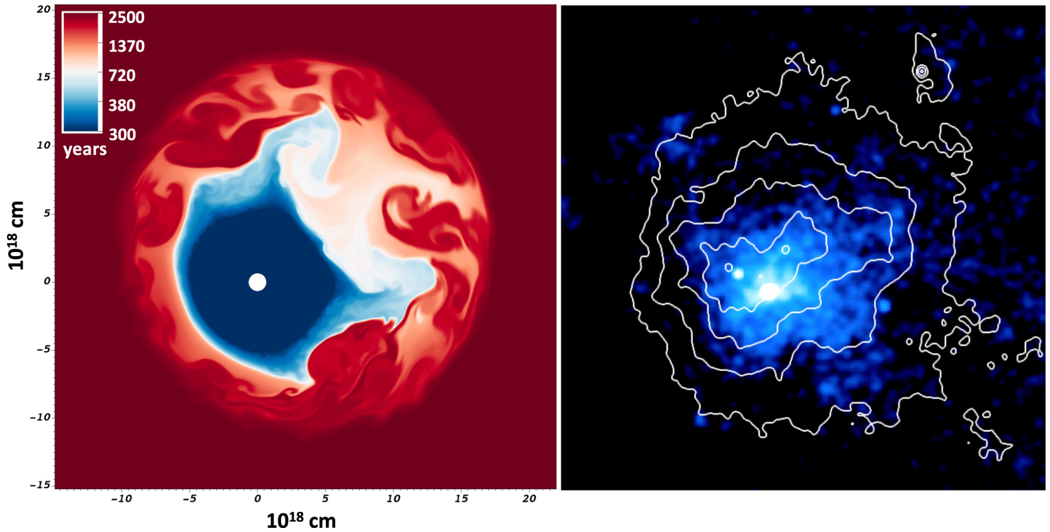
Figure 6. from Tea Temim et al 2022 Astrophys. J. 932 doi:10.3847/1538-4357/ac6bf4 https://dx.doi.org/10.3847/1538-4357/ac6bf4 © 2022. The Author(s). Published by the American Astronomical Society.
