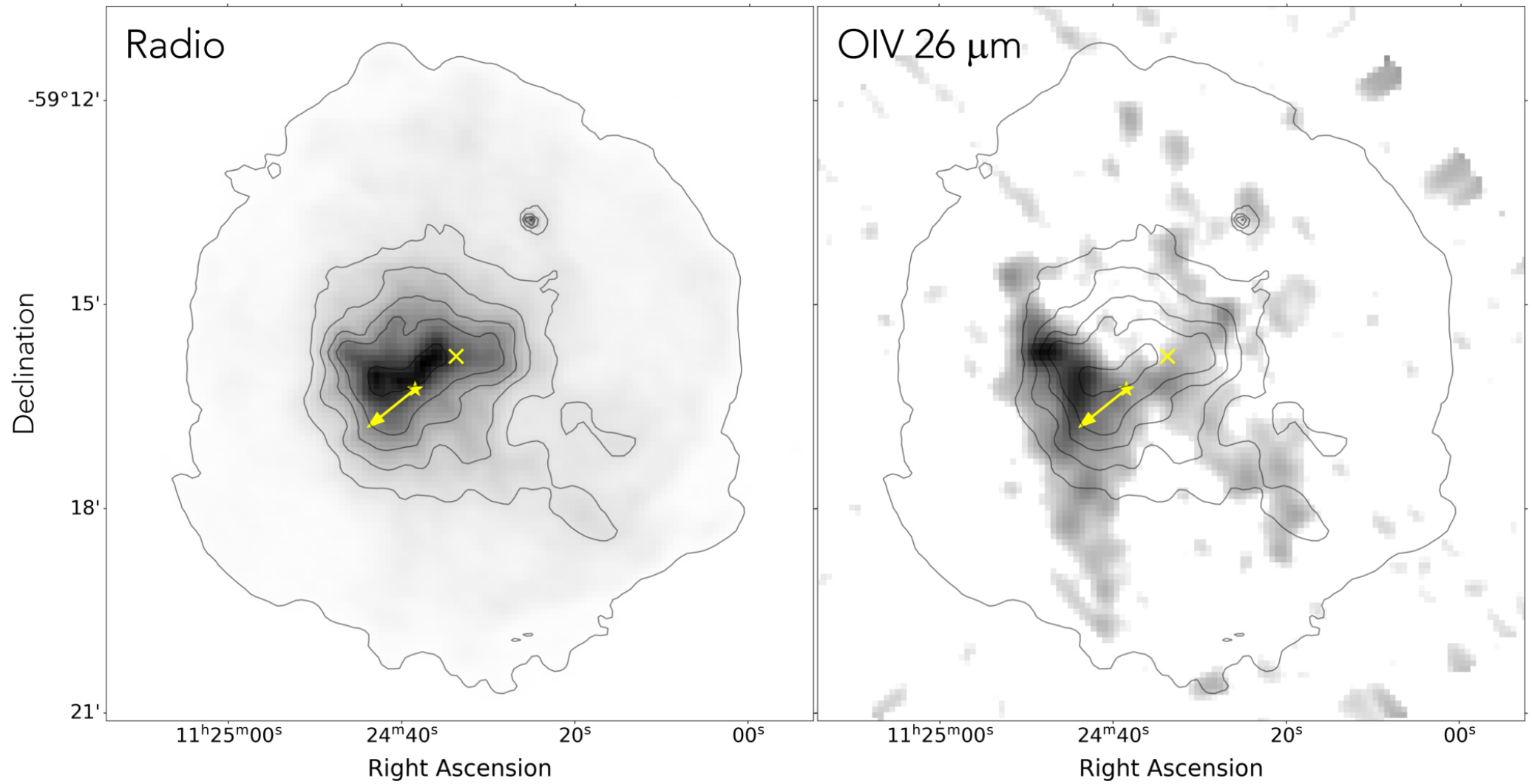
Figure 2. from Tea Temim et al 2022 Astrophys. J. 932 doi:10.3847/1538-4357/ac6bf4 https://dx.doi.org/10.3847/1538-4357/ac6bf4 © 2022. The Author(s). Published by the American Astronomical Society.
