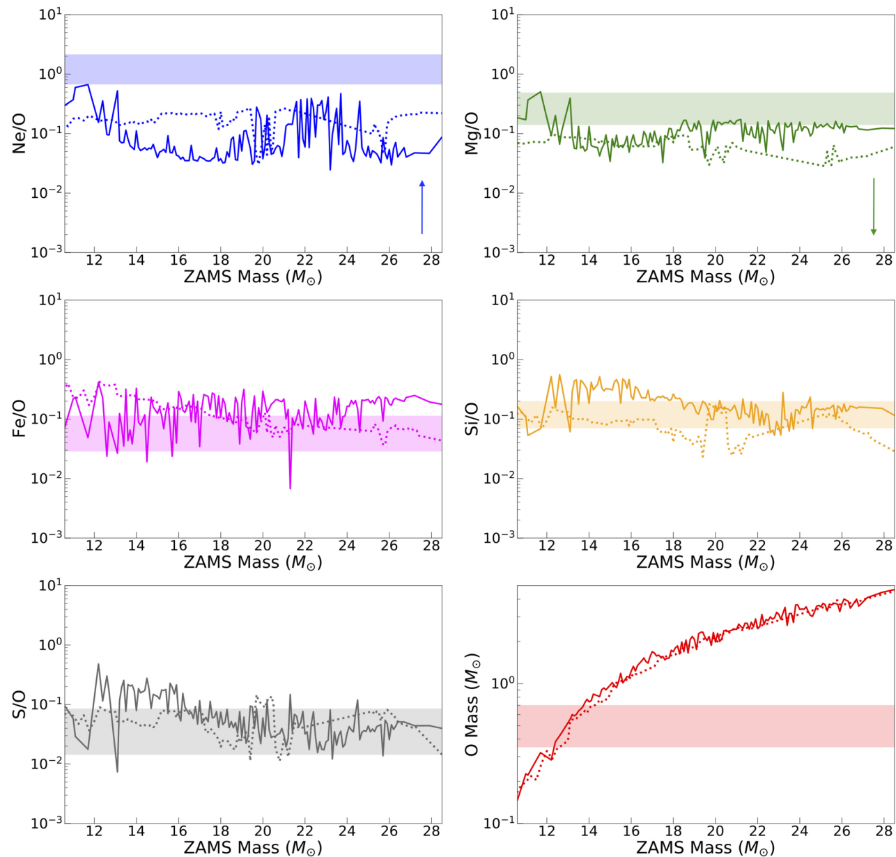
Figure 10. from Tea Temim et al 2022 Astrophys. J. 932 doi:10.3847/1538-4357/ac6bf4 https://dx.doi.org/10.3847/1538-4357/ac6bf4 © 2022. The Author(s). Published by the American Astronomical Society.
