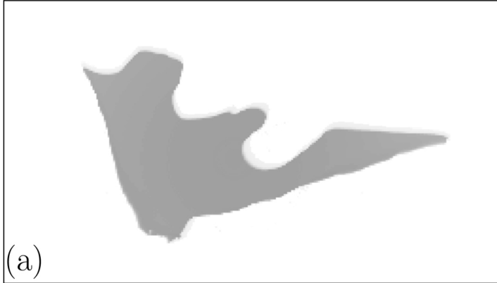
Figure 5. from V. Aslanyan et al 2022 Astrophys. J. 931 doi:10.3847/1538-4357/ac69ed https://dx.doi.org/10.3847/1538-4357/ac69ed © 2022. The Author(s). Published by the American Astronomical Society.
