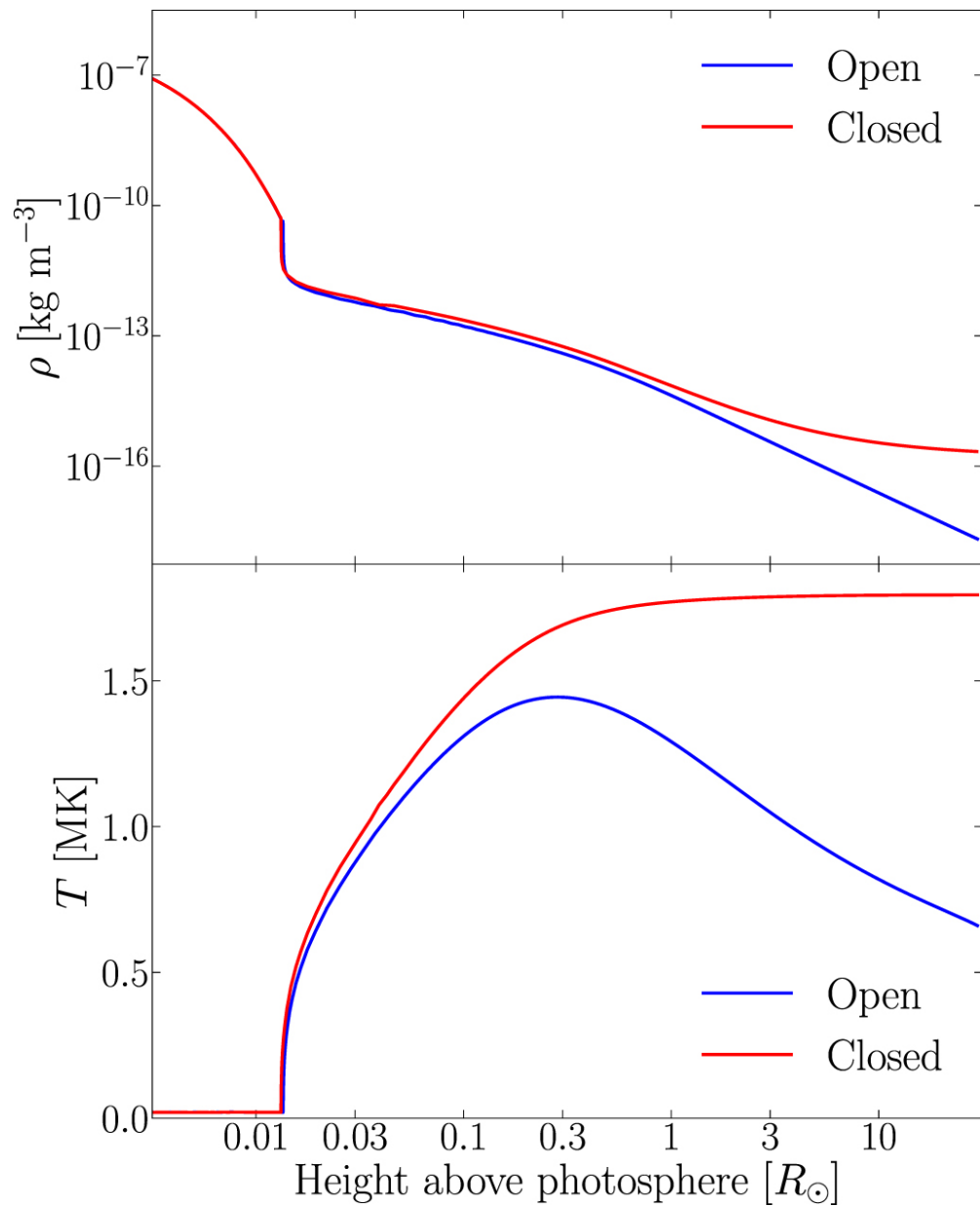
Figure 3. from V. Aslanyan et al 2022 Astrophys. J. 931 doi:10.3847/1538-4357/ac69ed https://dx.doi.org/10.3847/1538-4357/ac69ed © 2022. The Author(s). Published by the American Astronomical Society.
