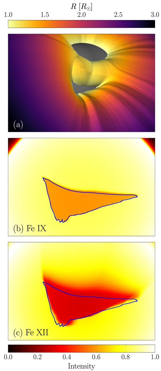
Figure 2. from V. Aslanyan et al 2022 Astrophys. J. 931 doi:10.3847/1538-4357/ac69ed https://dx.doi.org/10.3847/1538-4357/ac69ed © 2022. The Author(s). Published by the American Astronomical Society.
