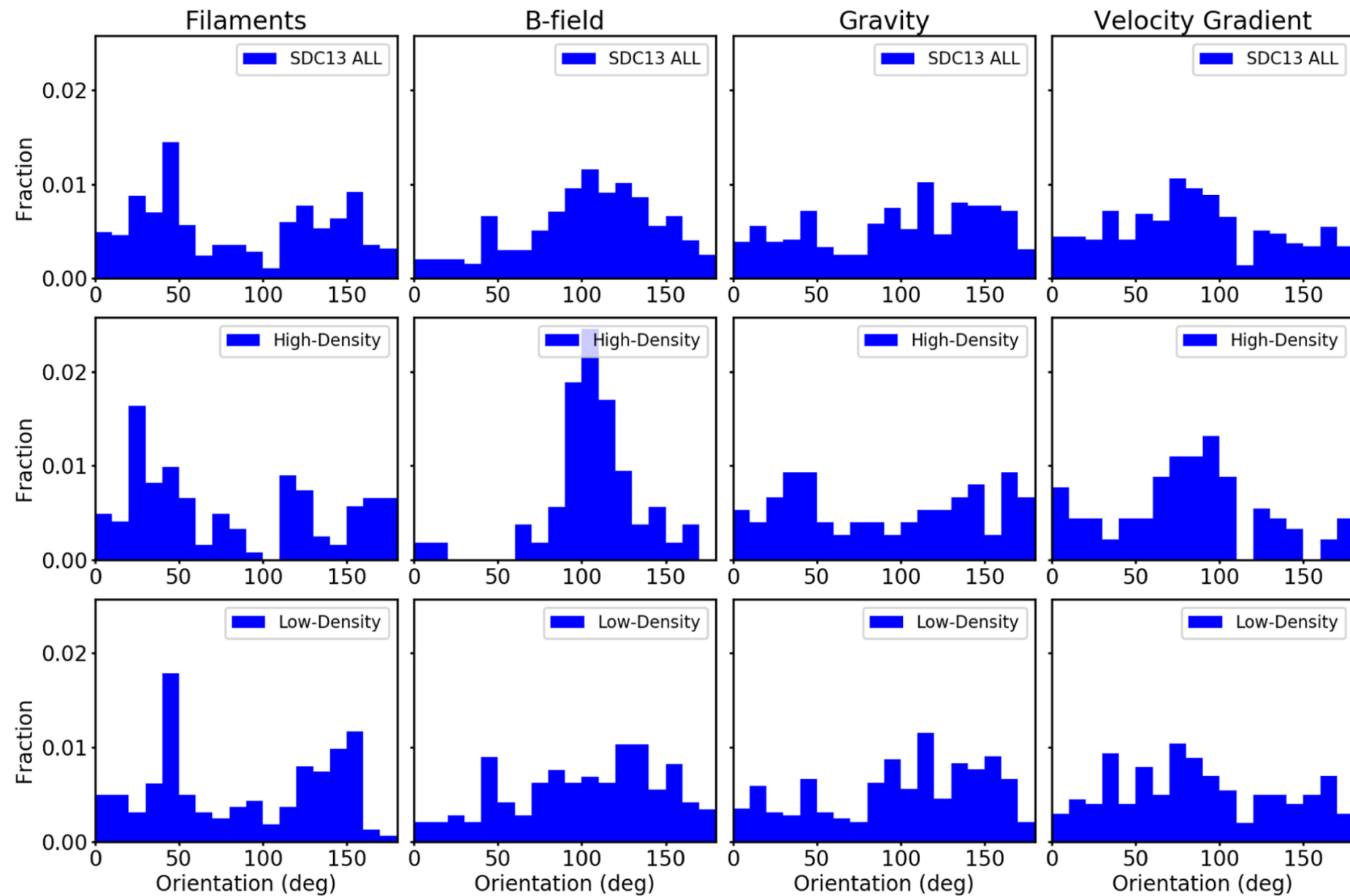
Figure 7. from Jia-Wei Wang et al 2022 Astrophys. J. 931 doi:10.3847/1538-4357/ac6872 https://dx.doi.org/10.3847/1538-4357/ac6872 © 2022. The Author(s). Published by the American Astronomical Society.
