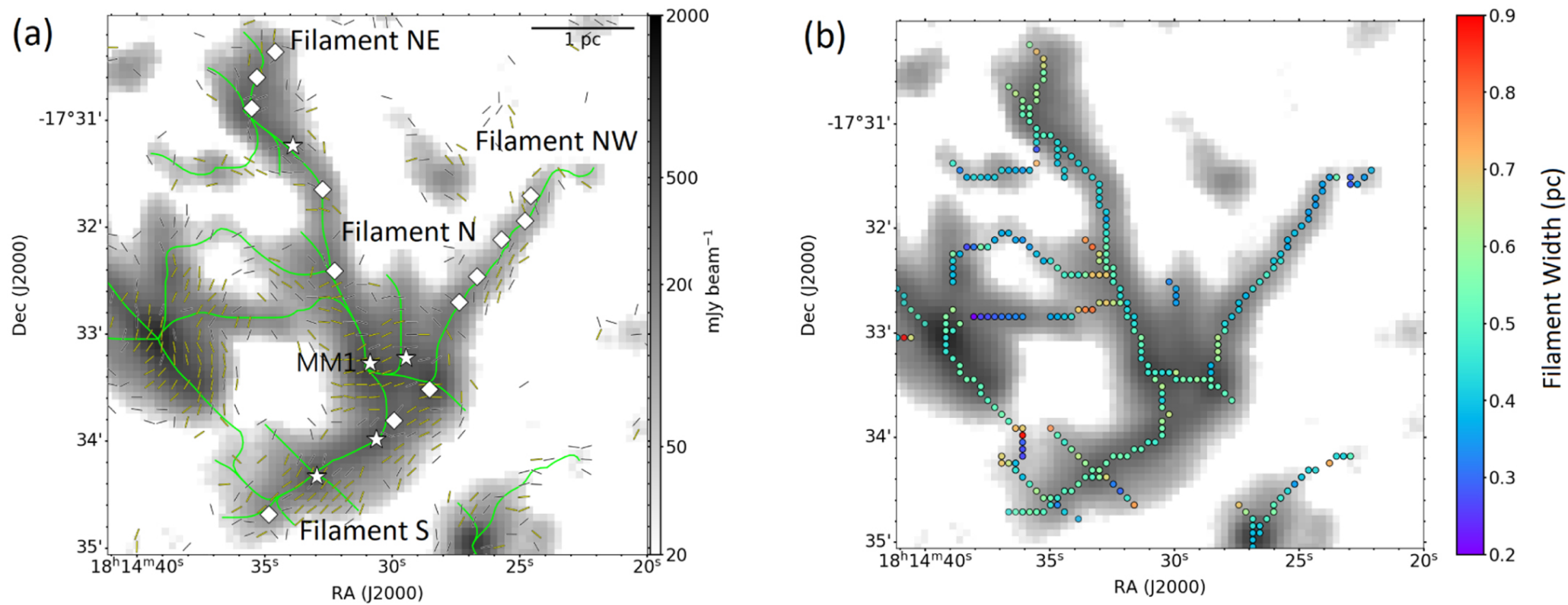
Figure 4. from Jia-Wei Wang et al 2022 Astrophys. J. 931 doi:10.3847/1538-4357/ac6872 https://dx.doi.org/10.3847/1538-4357/ac6872 © 2022. The Author(s). Published by the American Astronomical Society.
