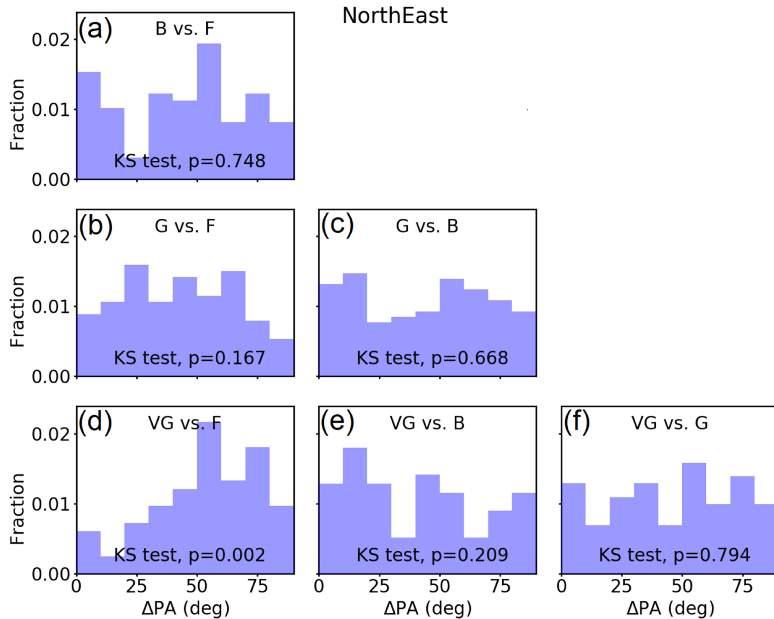
Figure 22. from Jia-Wei Wang et al 2022 Astrophys. J. 931 doi:10.3847/1538-4357/ac6872 https://dx.doi.org/10.3847/1538-4357/ac6872 © 2022. The Author(s). Published by the American Astronomical Society.
