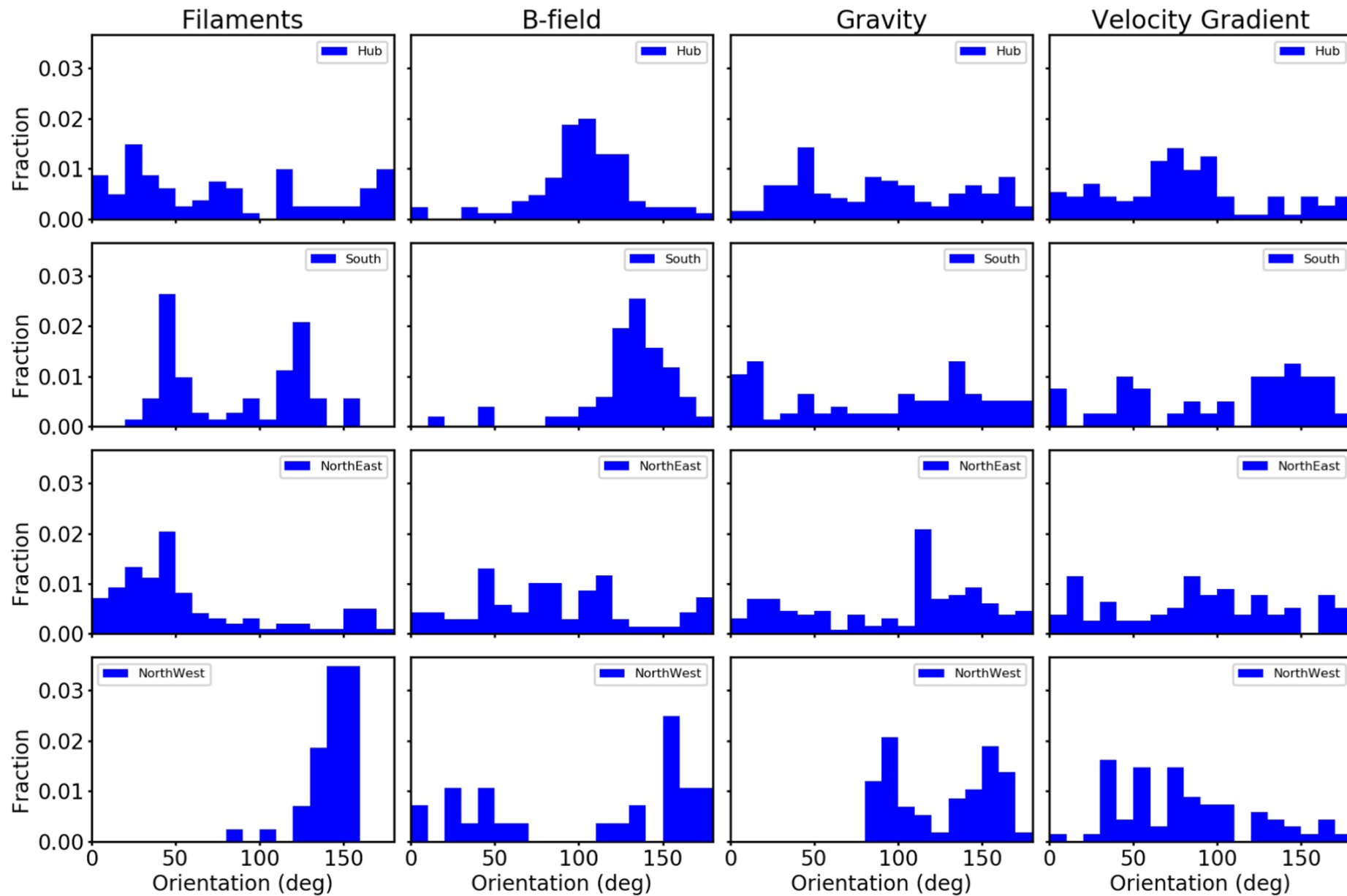
Figure 20. from Jia-Wei Wang et al 2022 Astrophys. J. 931 doi:10.3847/1538-4357/ac6872 https://dx.doi.org/10.3847/1538-4357/ac6872 © 2022. The Author(s). Published by the American Astronomical Society.
