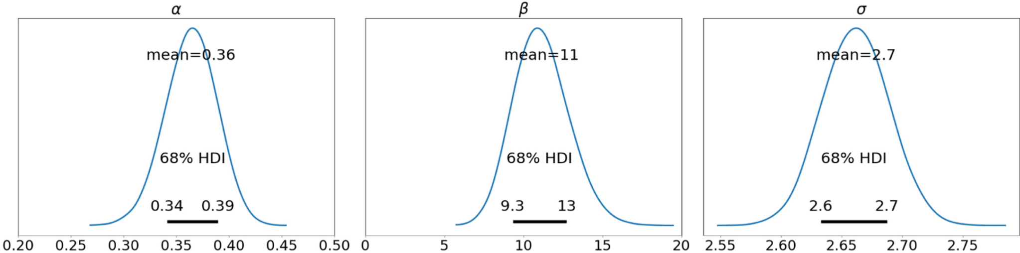
Figure 19. from Jia-Wei Wang et al 2022 Astrophys. J. 931 doi:10.3847/1538-4357/ac6872 https://dx.doi.org/10.3847/1538-4357/ac6872 © 2022. The Author(s). Published by the American Astronomical Society.
