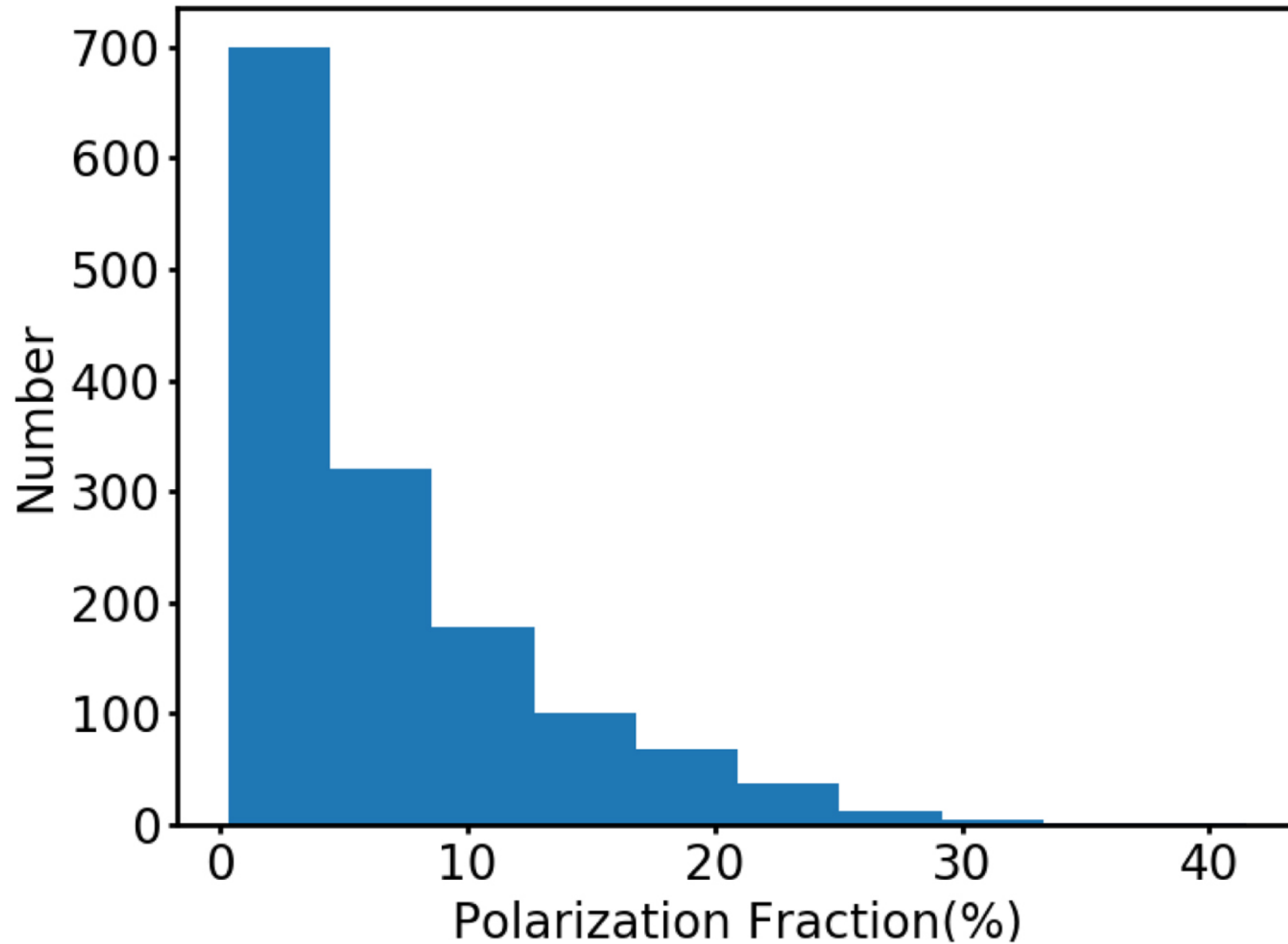
Figure 17. from Jia-Wei Wang et al 2022 Astrophys. J. 931 doi:10.3847/1538-4357/ac6872 https://dx.doi.org/10.3847/1538-4357/ac6872 © 2022. The Author(s). Published by the American Astronomical Society.
