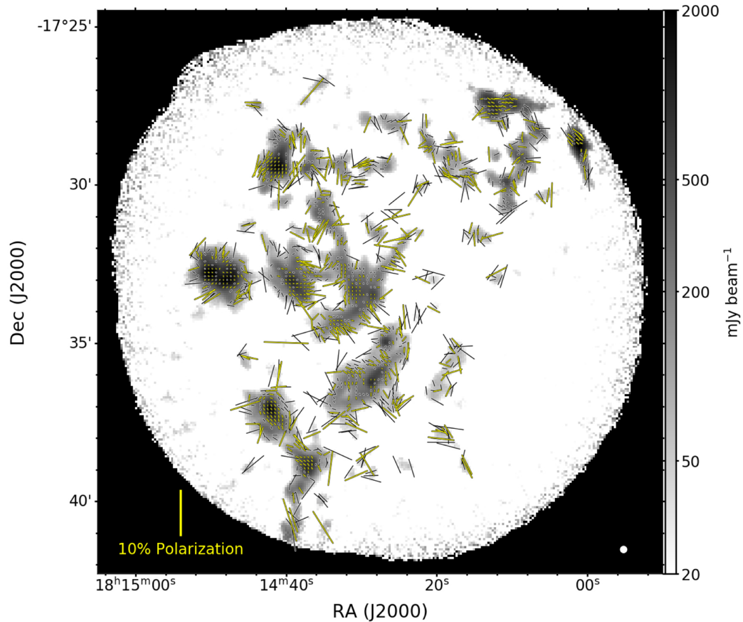
Figure 16. from Jia-Wei Wang et al 2022 Astrophys. J. 931 doi:10.3847/1538-4357/ac6872 https://dx.doi.org/10.3847/1538-4357/ac6872 © 2022. The Author(s). Published by the American Astronomical Society.
