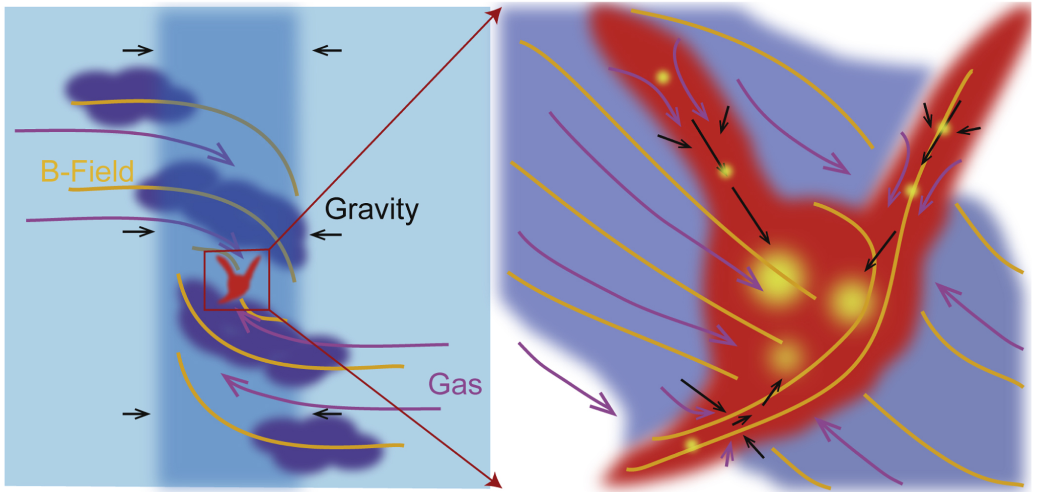
Figure 15. from Jia-Wei Wang et al 2022 Astrophys. J. 931 doi:10.3847/1538-4357/ac6872 https://dx.doi.org/10.3847/1538-4357/ac6872 © 2022. The Author(s). Published by the American Astronomical Society.
