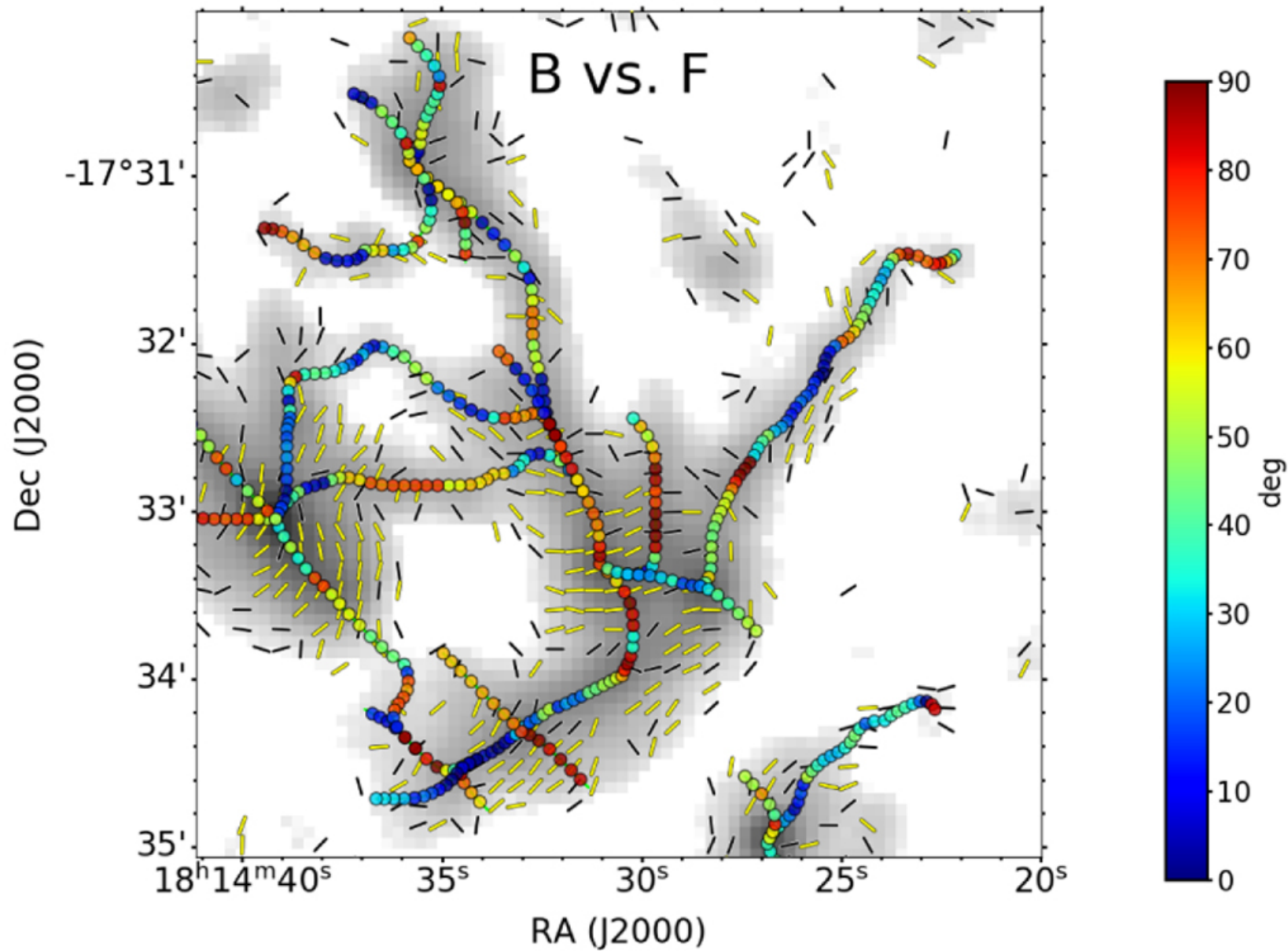
Figure 14. from Jia-Wei Wang et al 2022 Astrophys. J. 931 doi:10.3847/1538-4357/ac6872 https://dx.doi.org/10.3847/1538-4357/ac6872 © 2022. The Author(s). Published by the American Astronomical Society.
