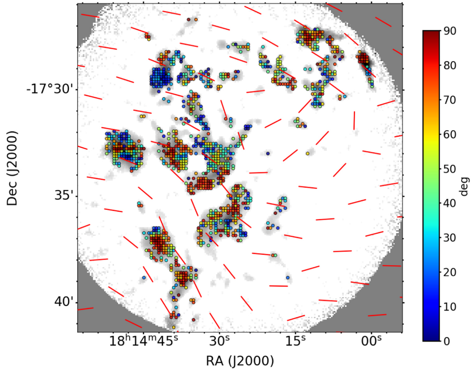
Figure 11. from Jia-Wei Wang et al 2022 Astrophys. J. 931 doi:10.3847/1538-4357/ac6872 https://dx.doi.org/10.3847/1538-4357/ac6872 © 2022. The Author(s). Published by the American Astronomical Society.
