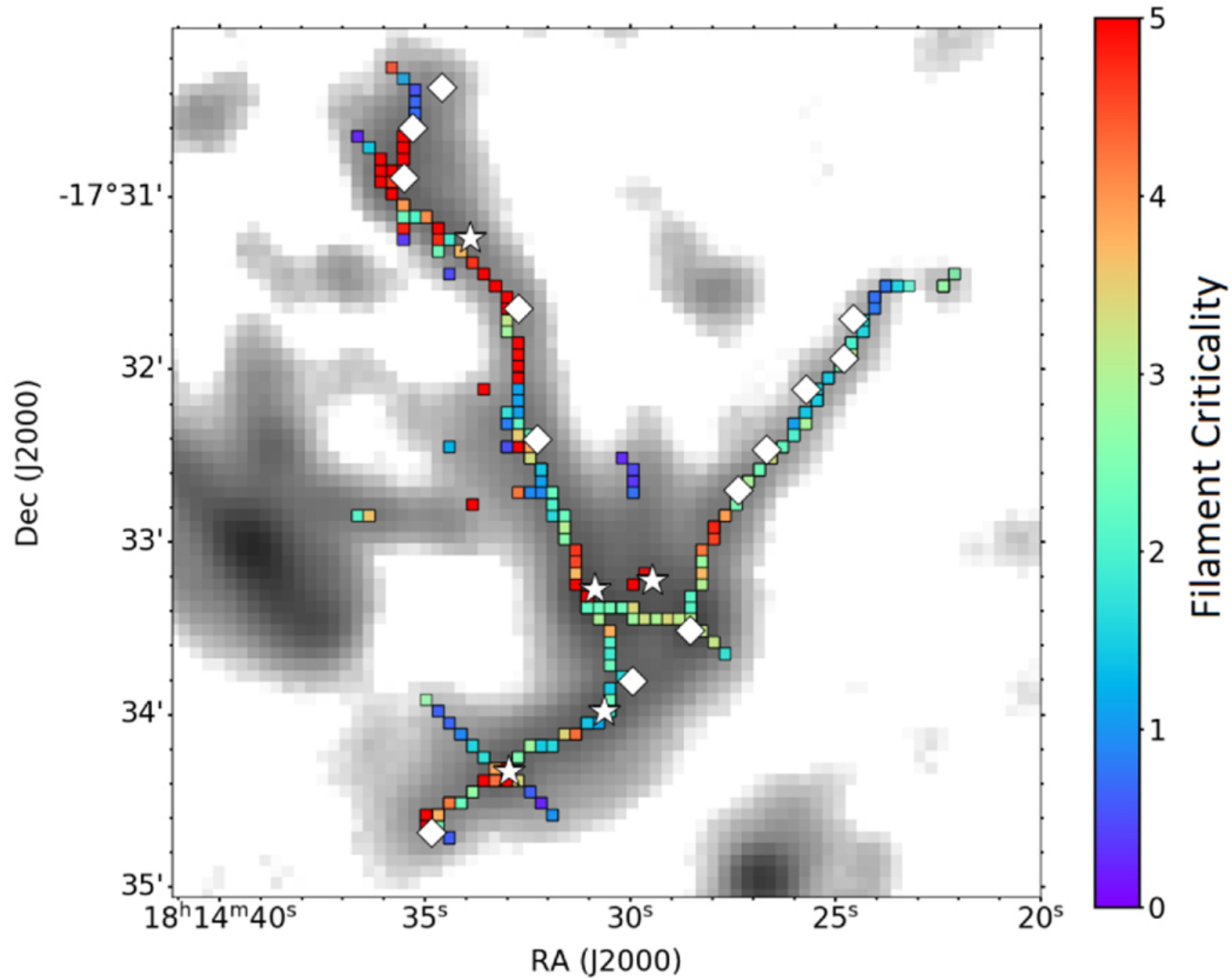
Figure 10. from Jia-Wei Wang et al 2022 Astrophys. J. 931 doi:10.3847/1538-4357/ac6872 https://dx.doi.org/10.3847/1538-4357/ac6872 © 2022. The Author(s). Published by the American Astronomical Society.
