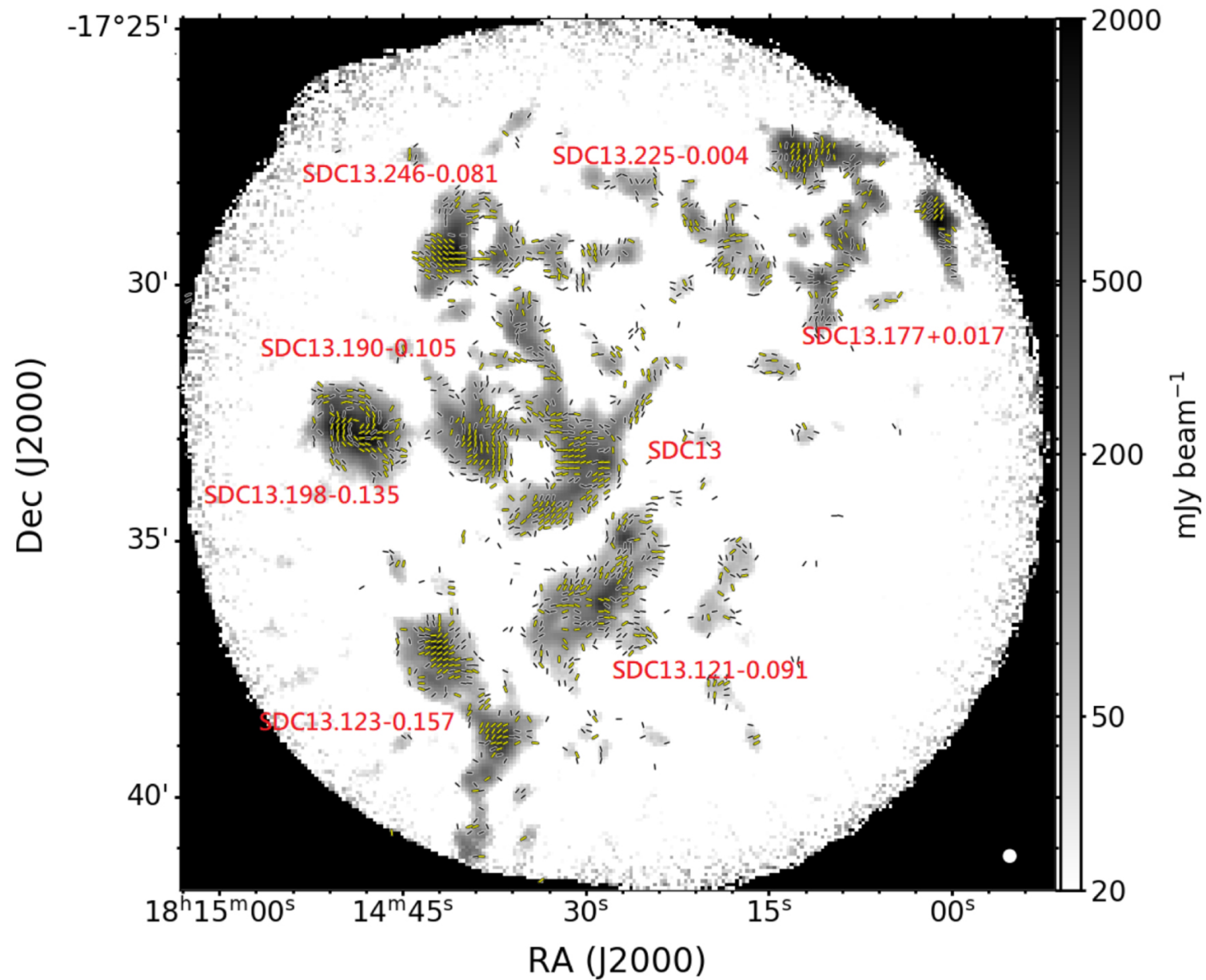
Figure 1. from Jia-Wei Wang et al 2022 Astrophys. J. 931 doi:10.3847/1538-4357/ac6872 https://dx.doi.org/10.3847/1538-4357/ac6872 © 2022. The Author(s). Published by the American Astronomical Society.
