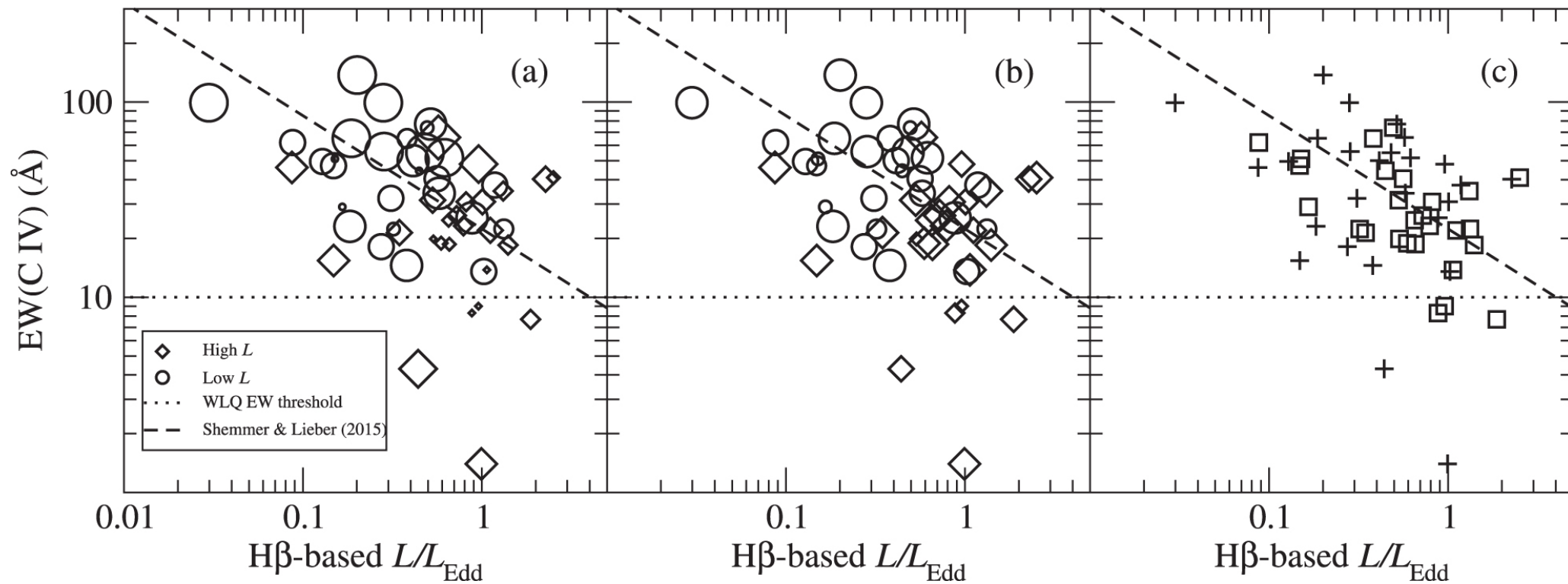
Figure 3. from Andrea Marlar et al 2022 Astrophys. J. 931 doi:10.3847/1538-4357/ac5f58 https://dx.doi.org/10.3847/1538-4357/ac5f58 © 2022. The Author(s). Published by the American Astronomical Society.
