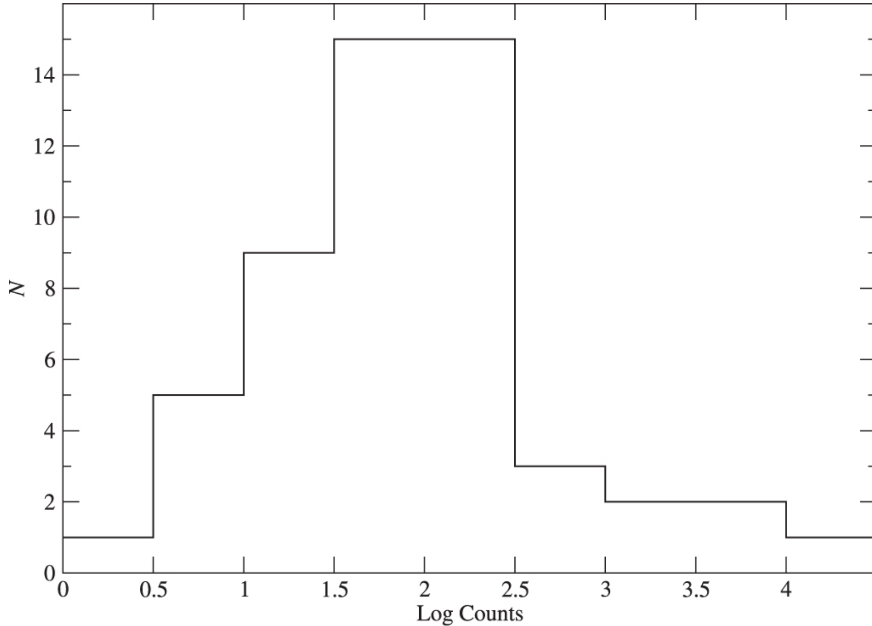
Figure 2. from Andrea Marlar et al 2022 Astrophys. J. 931 doi:10.3847/1538-4357/ac5f58 https://dx.doi.org/10.3847/1538-4357/ac5f58 © 2022. The Author(s). Published by the American Astronomical Society.
