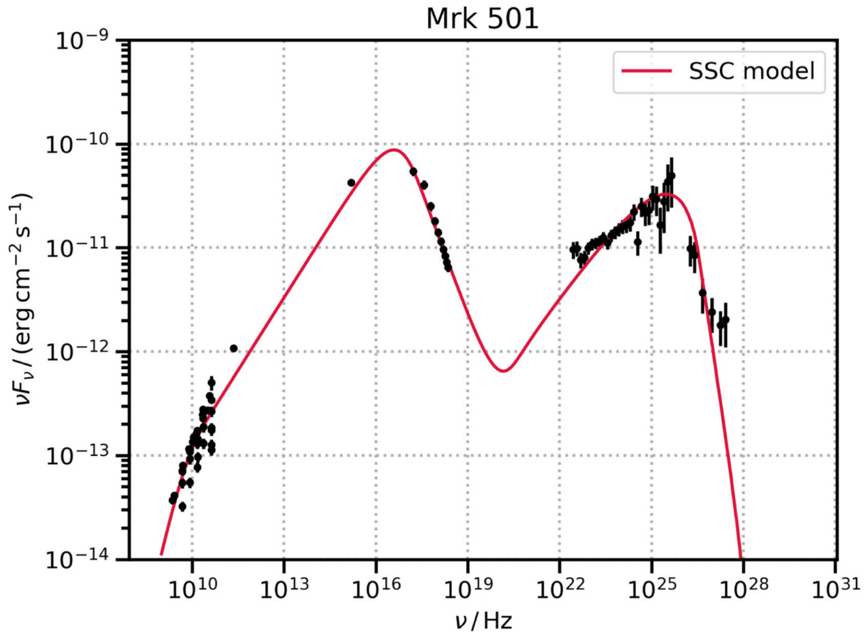
Figure 9. from A. Albert et al 2022 Astrophys. J. 929 doi:10.3847/1538-4357/ac58f6 https://dx.doi.org/10.3847/1538-4357/ac58f6 © 2022. The Author(s). Published by the American Astronomical Society.
