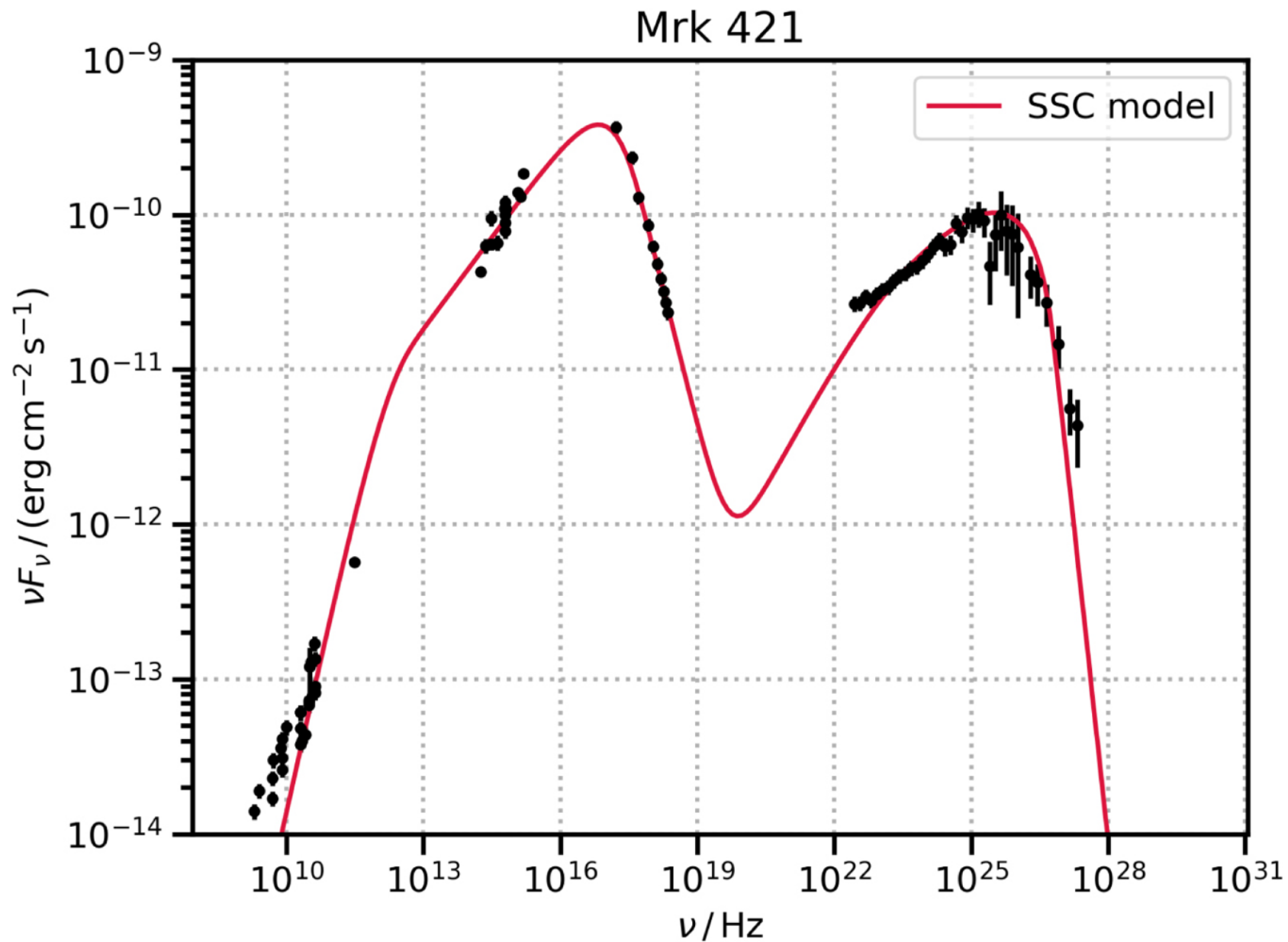
Figure 8. from A. Albert et al 2022 Astrophys. J. 929 doi:10.3847/1538-4357/ac58f6 https://dx.doi.org/10.3847/1538-4357/ac58f6 © 2022. The Author(s). Published by the American Astronomical Society.
