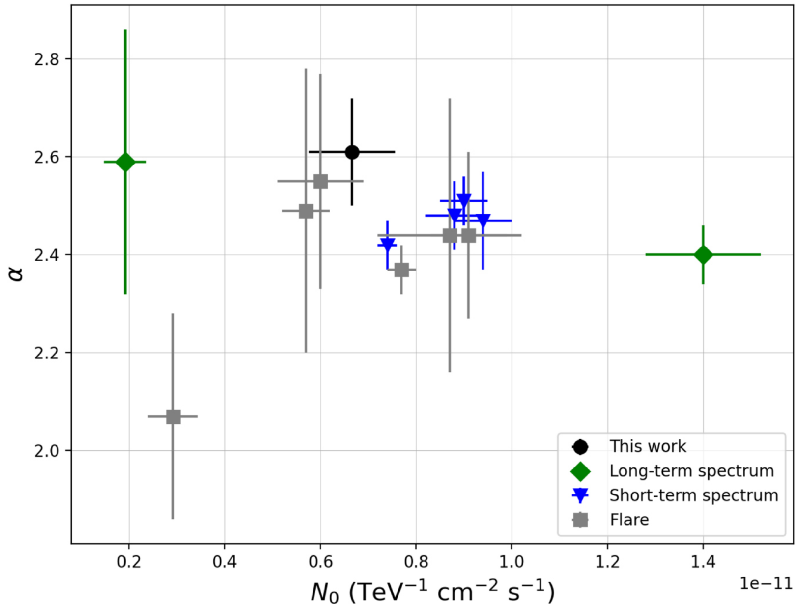
Figure 6. from A. Albert et al 2022 Astrophys. J. 929 doi:10.3847/1538-4357/ac58f6 https://dx.doi.org/10.3847/1538-4357/ac58f6 © 2022. The Author(s). Published by the American Astronomical Society.
