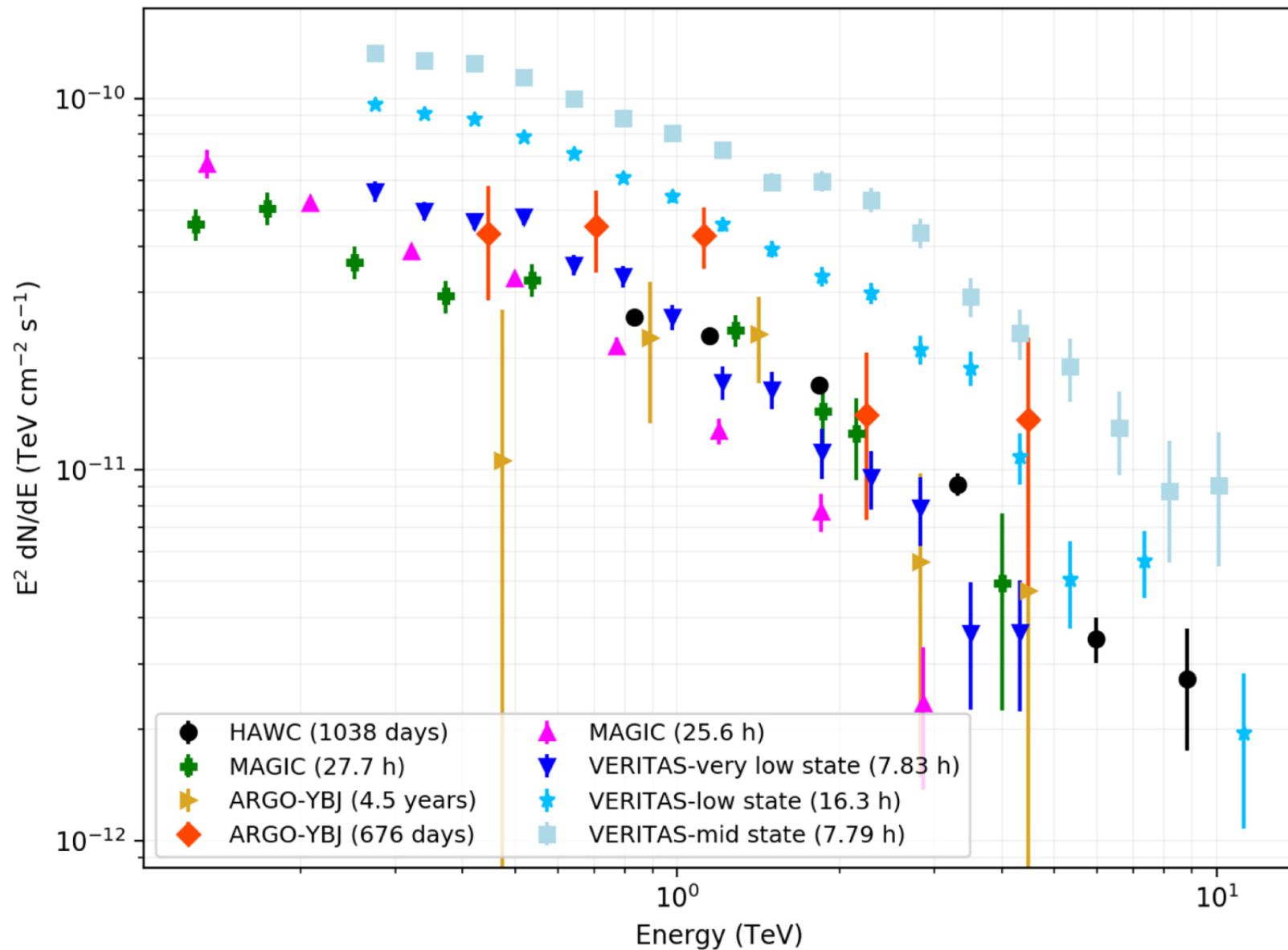
Figure 5. from A. Albert et al 2022 Astrophys. J. 929 doi:10.3847/1538-4357/ac58f6 https://dx.doi.org/10.3847/1538-4357/ac58f6 © 2022. The Author(s). Published by the American Astronomical Society.
