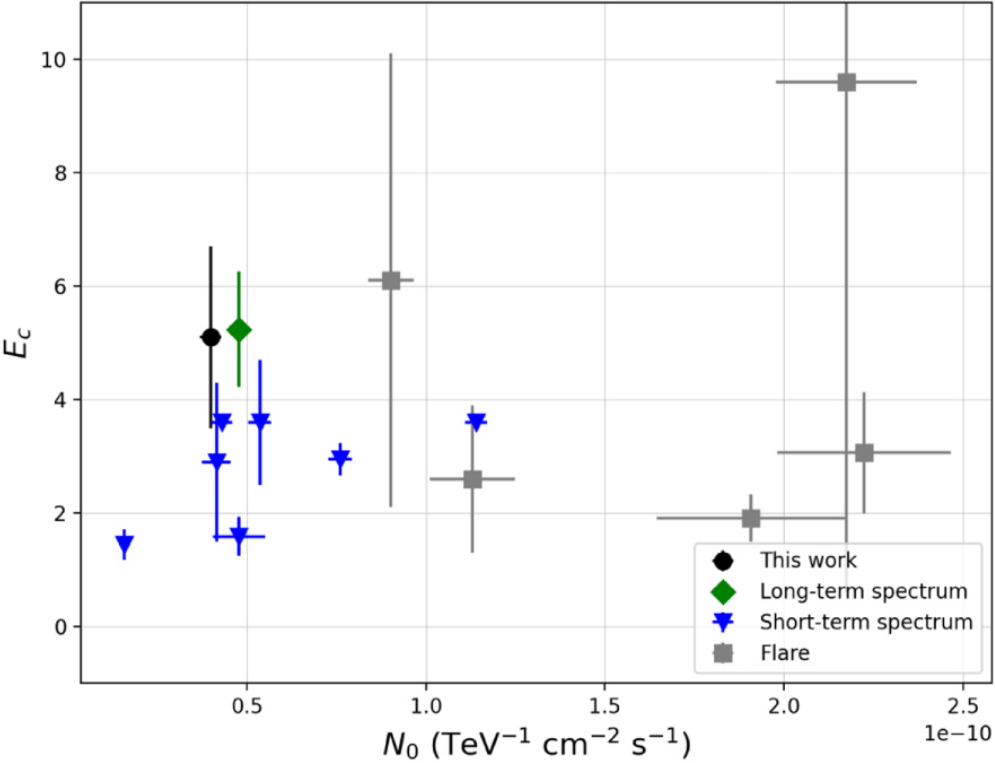
Energy cut-off vs. Normalization flux
