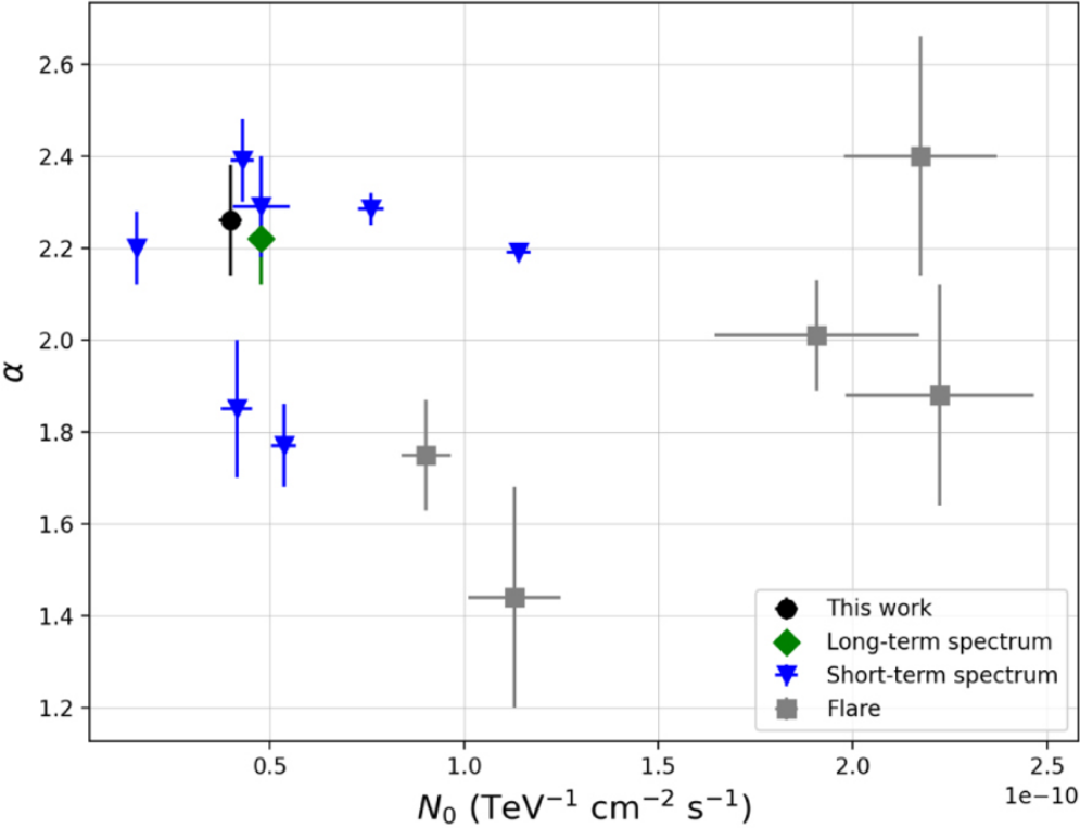
Figure 4. from A. Albert et al 2022 Astrophys. J. 929 doi:10.3847/1538-4357/ac58f6 https://dx.doi.org/10.3847/1538-4357/ac58f6 © 2022. The Author(s). Published by the American Astronomical Society.
