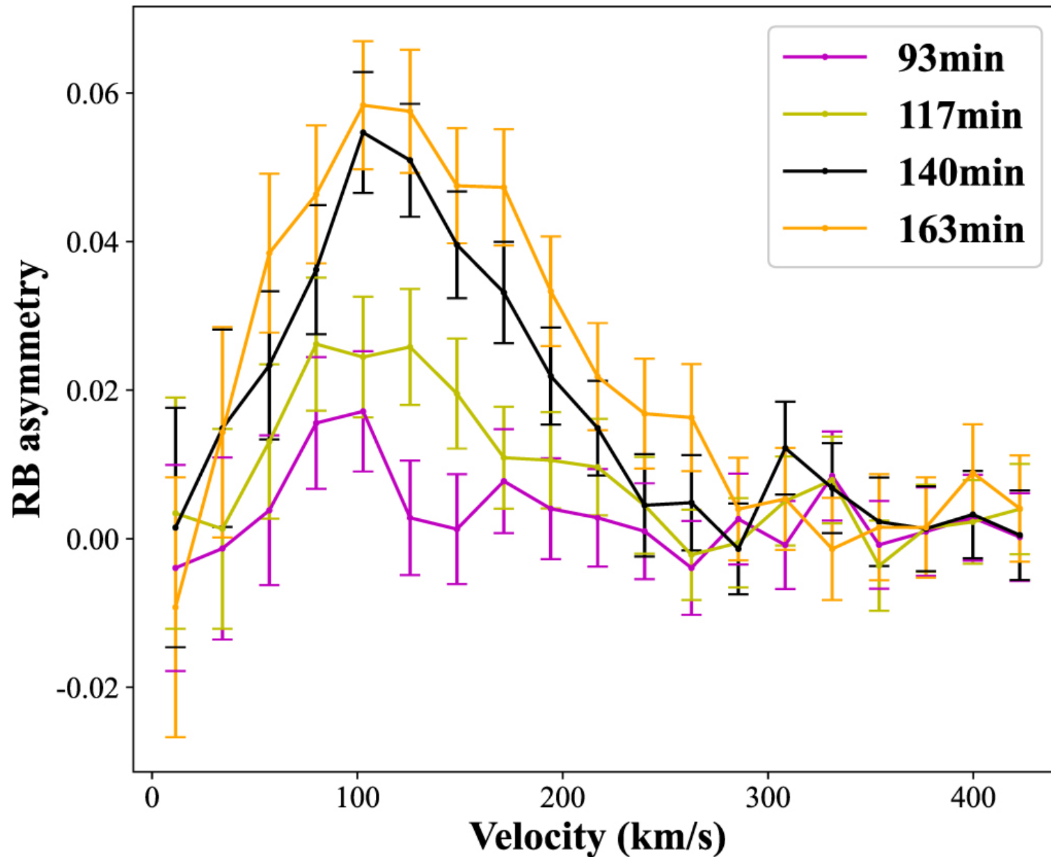
Figure 6. from Yuchuan Wu et al 2022 Astrophys. J. 928 doi:10.3847/1538-4357/ac5897 https://dx.doi.org/10.3847/1538-4357/ac5897 © 2022. The Author(s). Published by the American Astronomical Society.
