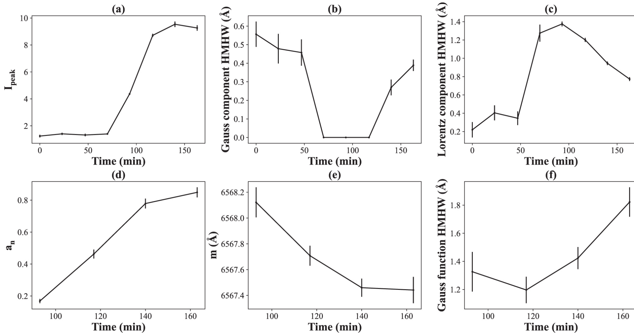
Figure 4. from Yuchuan Wu et al 2022 Astrophys. J. 928 doi:10.3847/1538-4357/ac5897 https://dx.doi.org/10.3847/1538-4357/ac5897 © 2022. The Author(s). Published by the American Astronomical Society.
